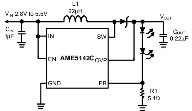
Figure 1: Circuit For Driving 2 White LEDs
