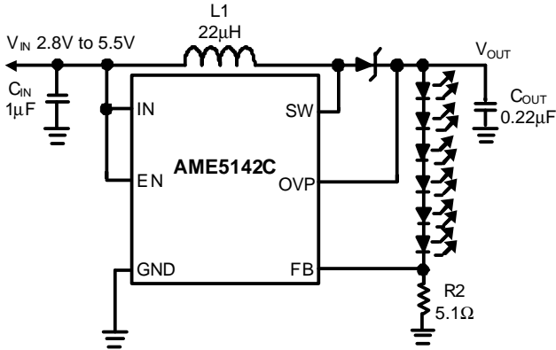
Figure 8: Circuit For Driving 6 White LEDs
