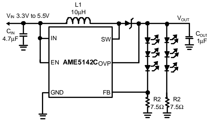
Figure 9: Circuit For Driving 2 Strings of 3 White LEDs
