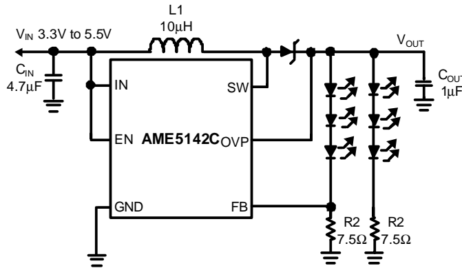
Figure 10: Circuit For Driving 2 Strings of 3 White LEDs
