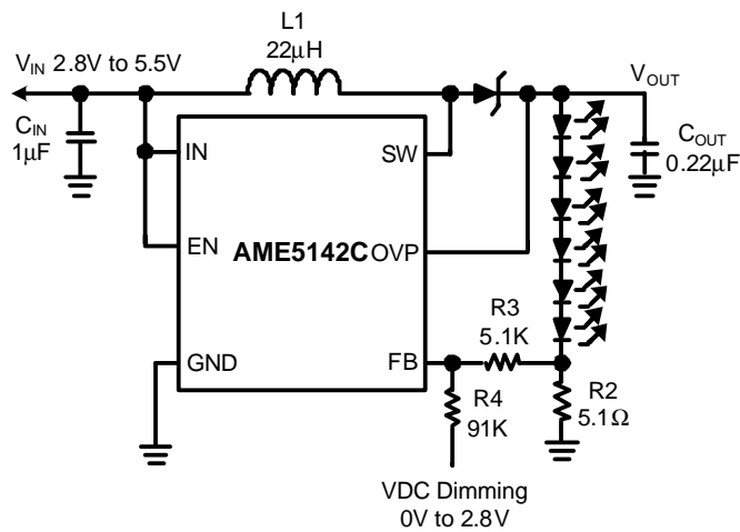
Figure 6. Dimming Control Using a DC Voltage
