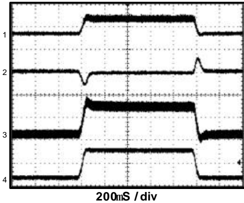
Load Step
