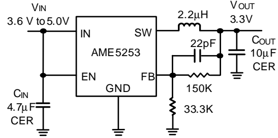
Figure 9: 3.3V Step-Down Regulator
