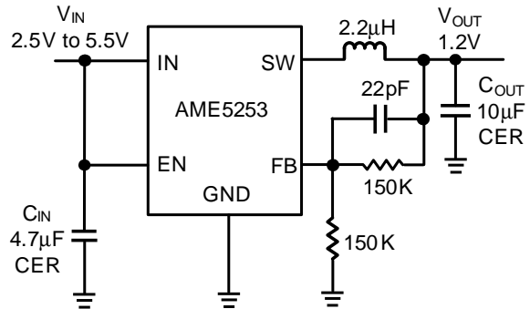
Figure 5: 1.2V Step-Down Regulator
