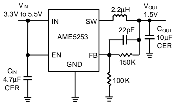
Figure 6: 1.5V Step-Down Regulator
