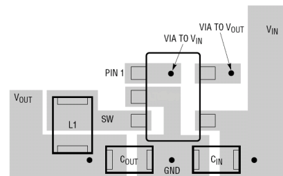
Figure 11: AME5253 Fixed Voltage Regulator Layout Diagram
