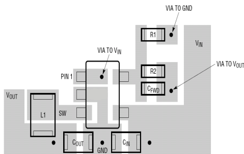
Figure 10: AME5253 Adjustable Voltage Regulator Layout Diagram
