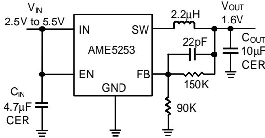
Figure 8: 1.6V Step-Down Regulator
