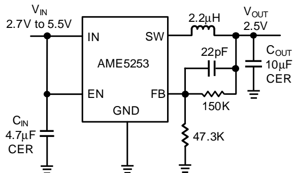
Figure 7: 2.5V Step-Down Regulator
