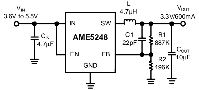
Figure 7. AME5248 with 3.3V Output
