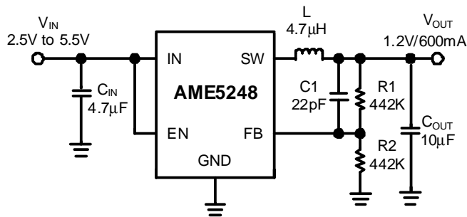
Figure 4. AME5248 with 1.2V Output
