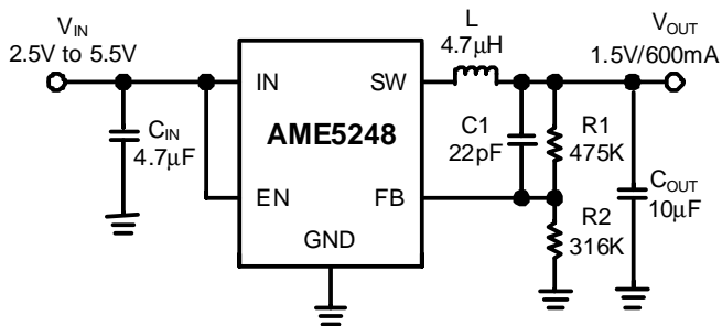
Figure 5. AME5248 with 1.5V Output
