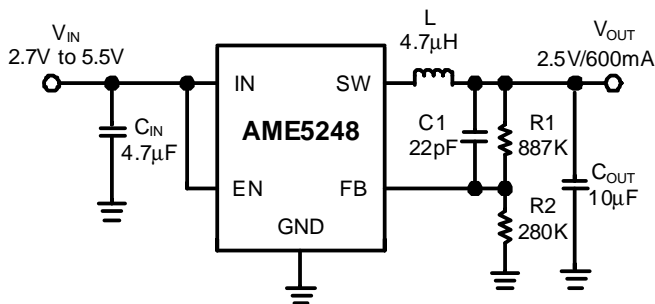
Figure 6. AME5248 with 2.5V Output
