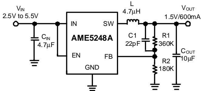
Figure 5. AME5248A with 1.5V Output
