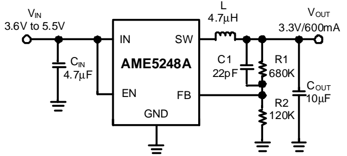
Figure 7. AME5248A with 3.3V Output
