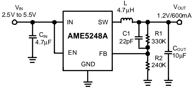
Figure 4. AME5248A with 1.2V Output
