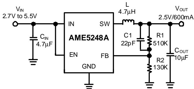
Figure 6. AME5248A with 2.5V Output
