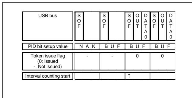
Figure 2.1 Token issue flag when "IITV=0"
