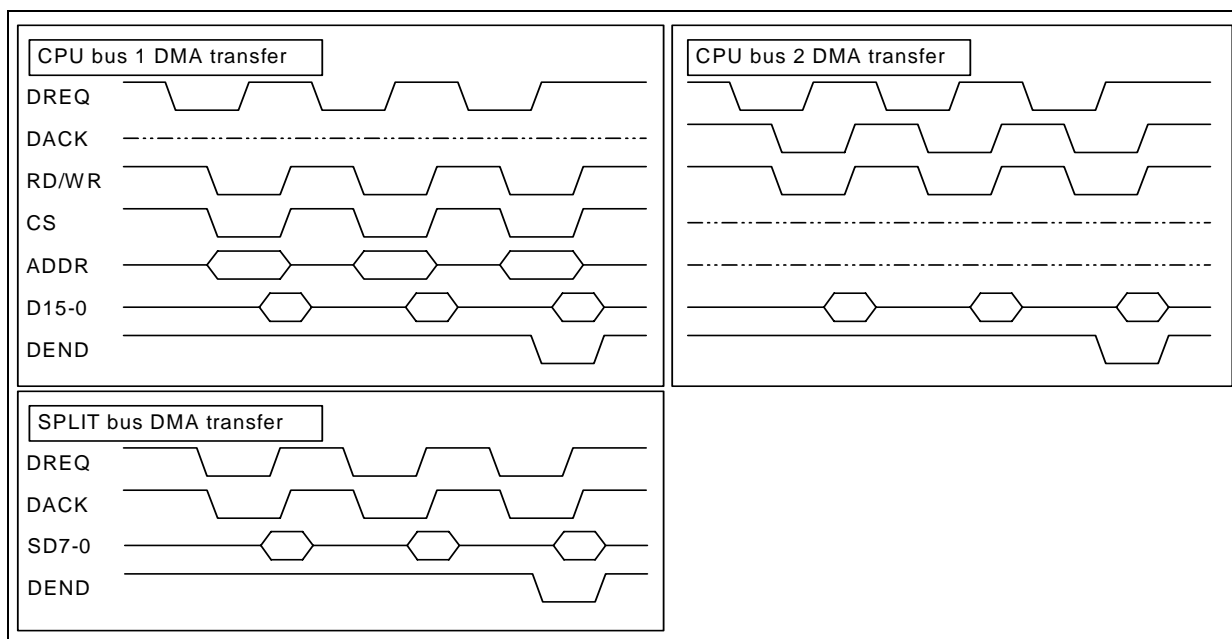
Figure 3.16 FIFO Port Access and DMA Control Pin
