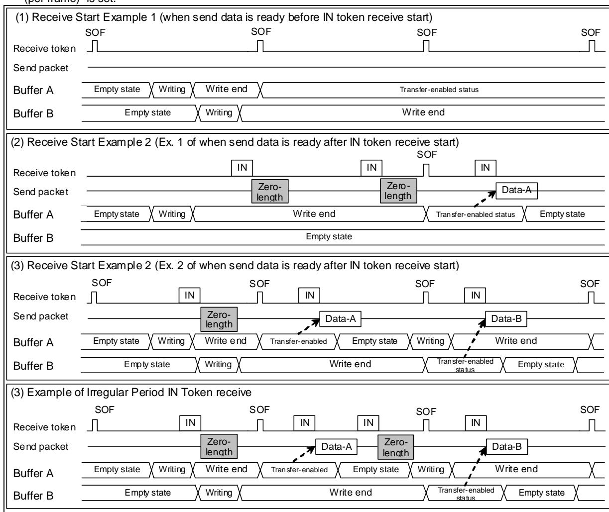
Figure 3.20 Data Setup Function Operation
