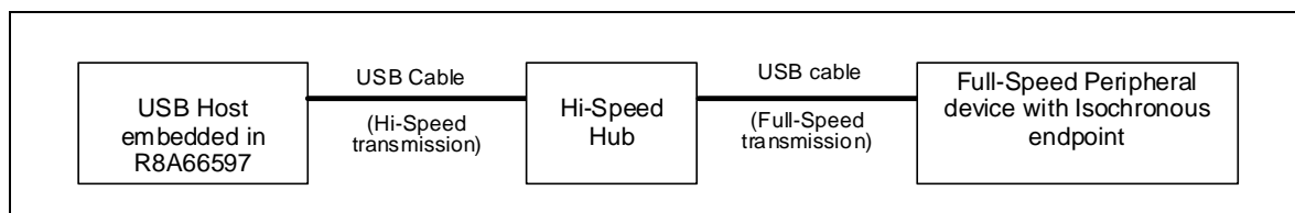
Figure 3.23 Connection Example of Split-Transaction Transfer
