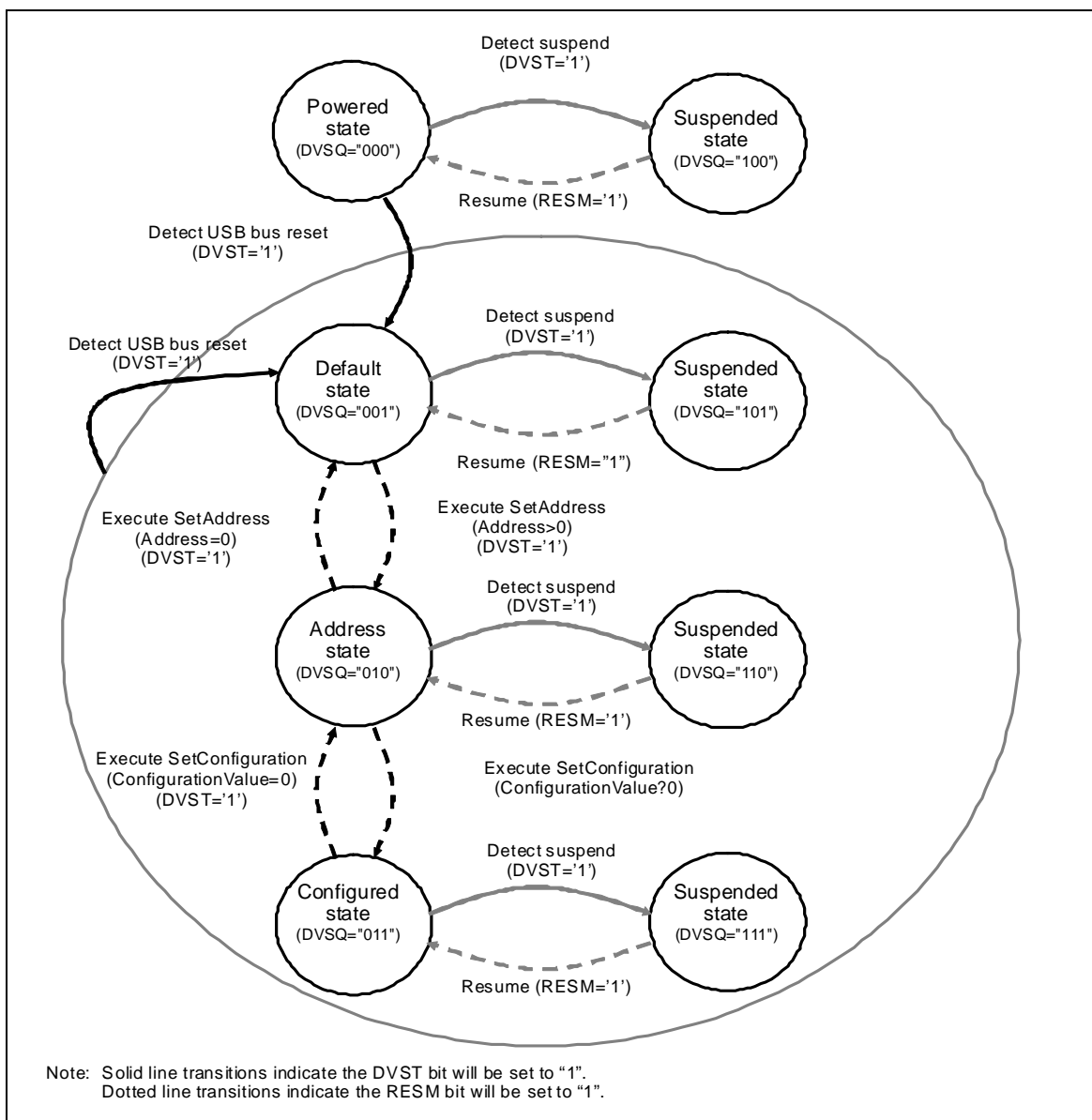
Figure 3.10 Device State Transitions
