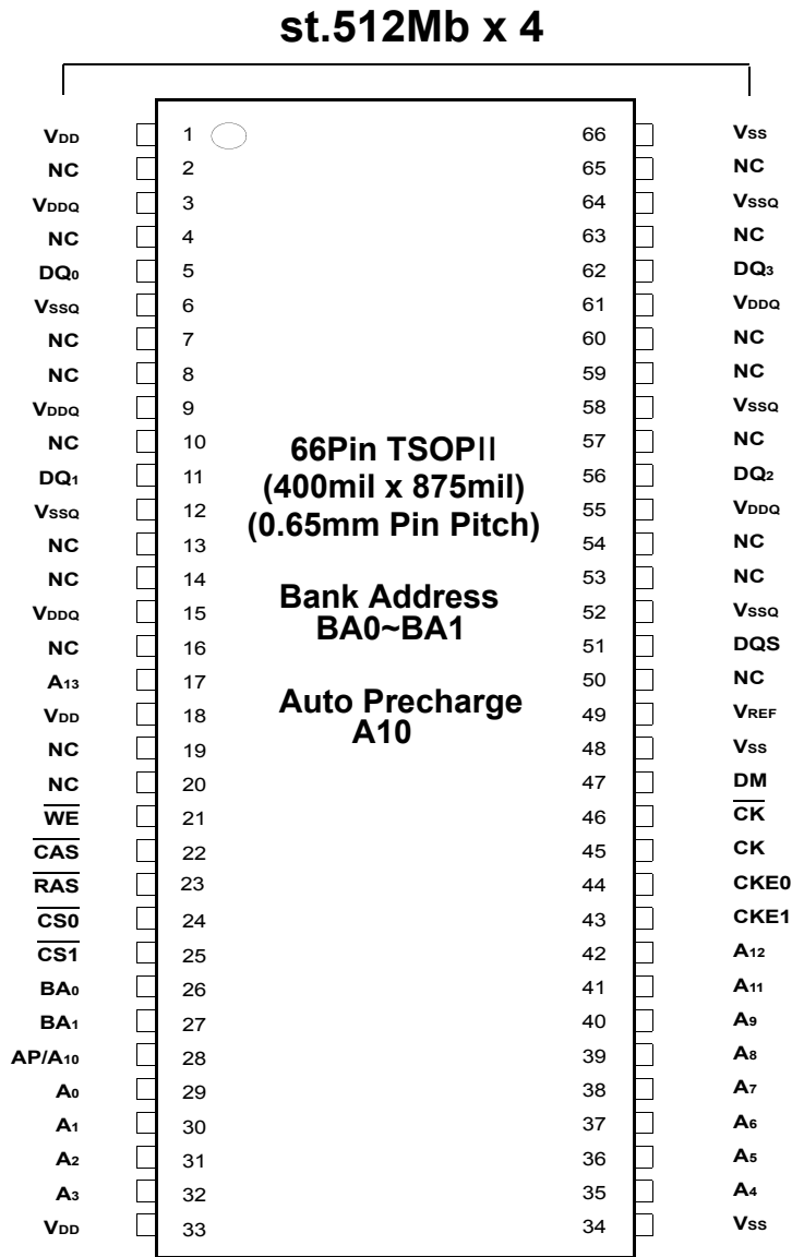
stacked 2Gb TSOP-II Package Pinout
