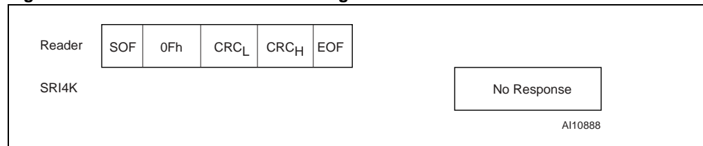
Figure 59. COMPLETION frame exchange between Reader and SRI4K
