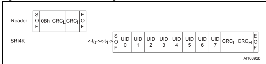
Figure 63. GET_UID frame exchange between Reader and SRI4K
