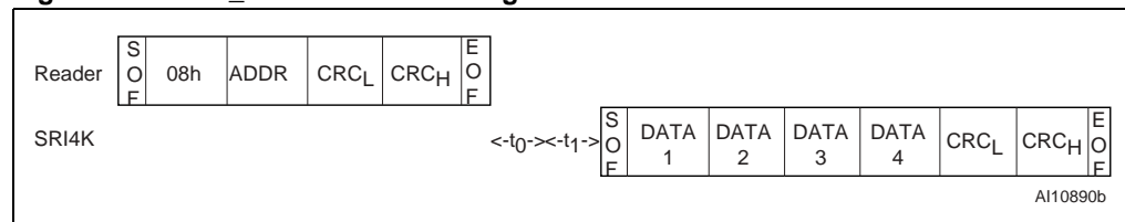
Figure 43. read_block frame exchange between reader and SRI4K
