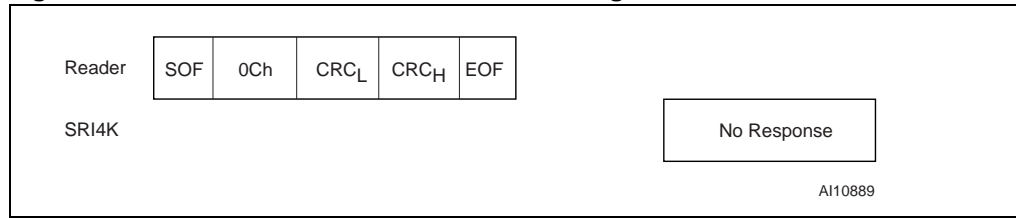
Figure 61. READ_BLOCK frame exchange between Reader and SRI4K
