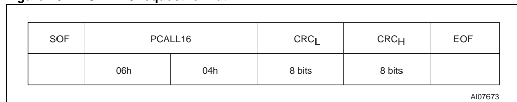
Figure 26. PCALL16 request format
