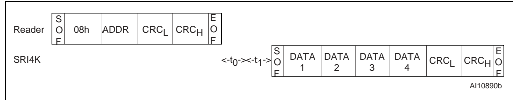
Figure 62. WRITE_BLOCK frame exchange between Reader and SRI4K
