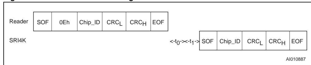
Figure 58. SELECT frame exchange between Reader and SRI4K
