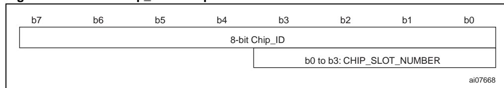
Figure 20. SRI4K Chip_ID description
