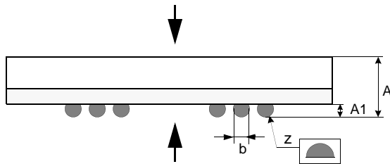
*1: Bottom View
