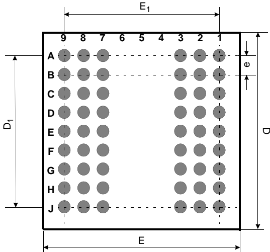
< Bottom View *1 >
