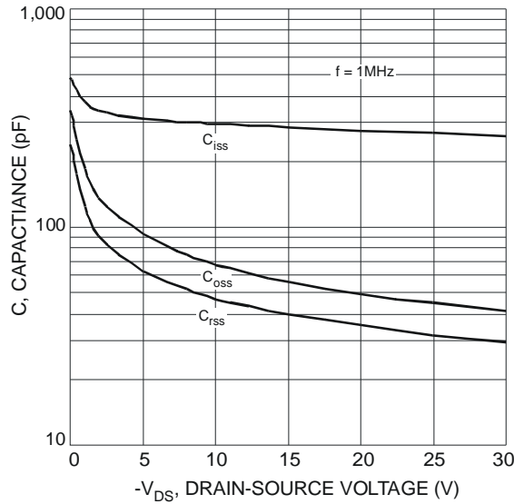
Fig. 6 Typical Capacitance
