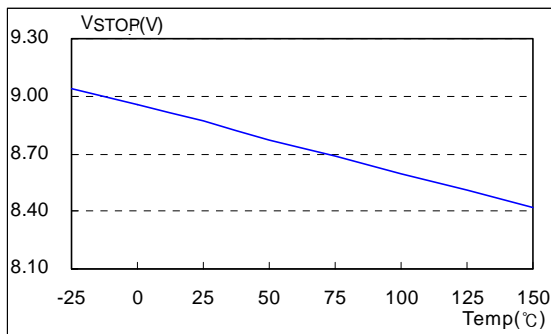
Figure 3. Stop Threshold Voltage vs. Temp
