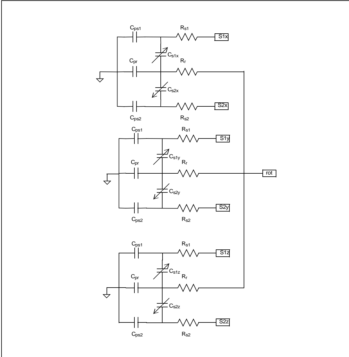
Figure 1. Equivalent electrical circuit
