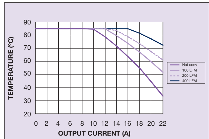
Figure 12 - Safe Operating Curve PTH05020W V_{out} = 3.3V
