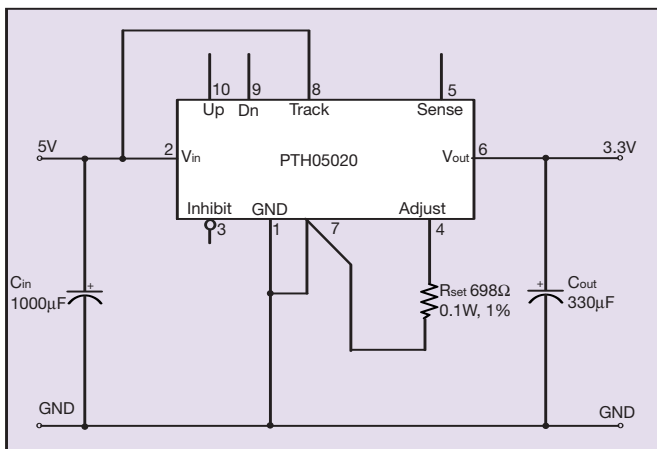
Figure 6 - Soft-Start Power-up
