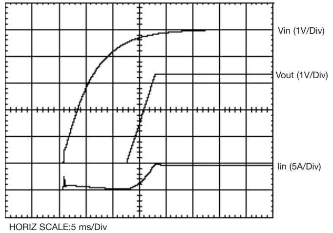
Figure 7 - Power-up Characteristic
