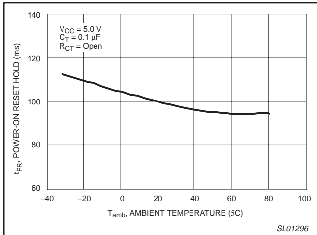
Figure 11. Power-on reset hold time versus temperature.
