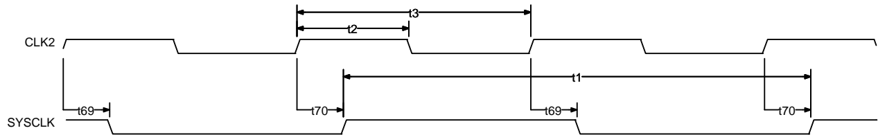
Figure 1) CLK2 to SYSCLK Skew
