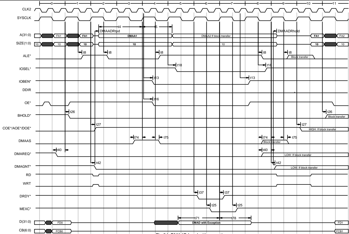
Fig 34: DMA IO Load with exception
