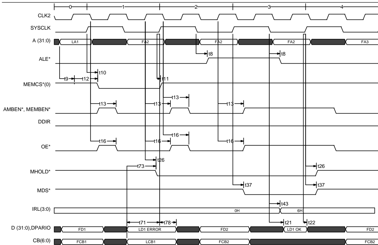
Figure 5) RAM Load at 0 waitstate with Correctable Error
