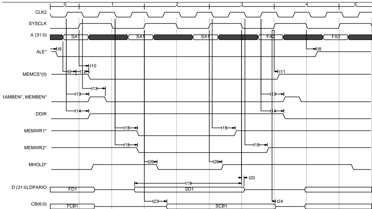
Figure 4) RAM Store at 1 waitstate with EDAC and/or Parity Protection
