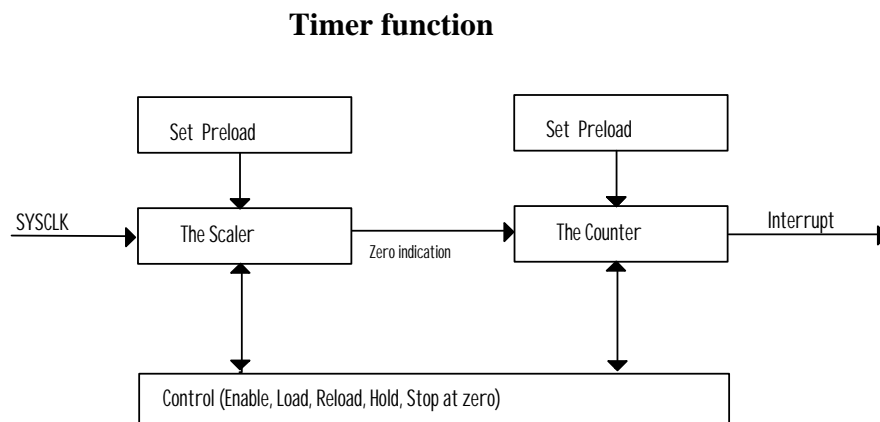
Figure 6 - Timer implementation
