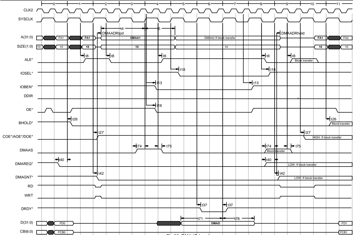
Fig 32: DMA IO Load
