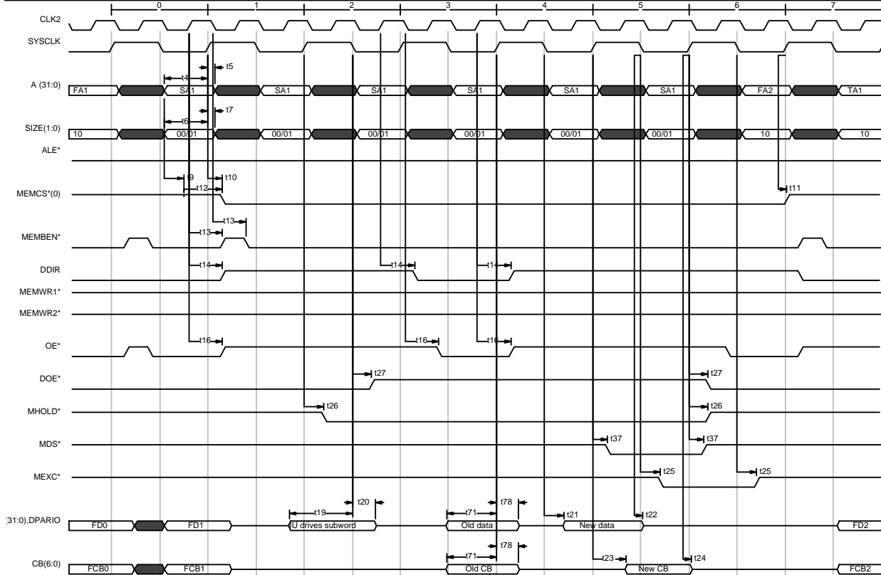
Figure 11) RAM Store Byte/Halfword with Uncorrectable Error
