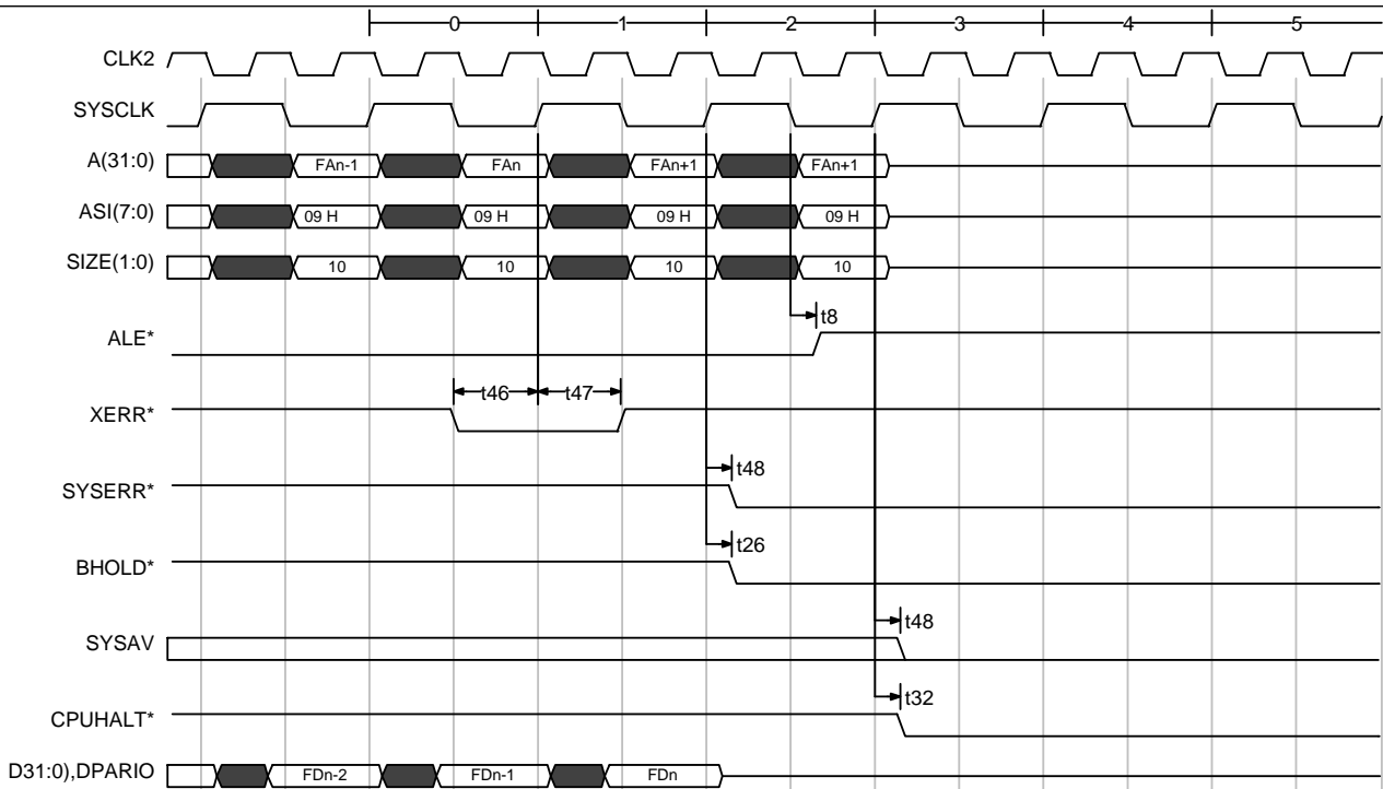
Fig 42) External Error with Halt Timing
