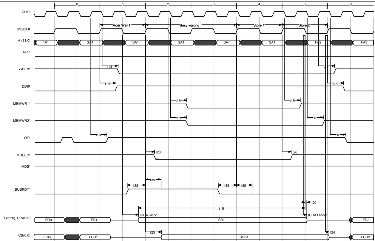
Fig 29) Extended Area Store with Busy
