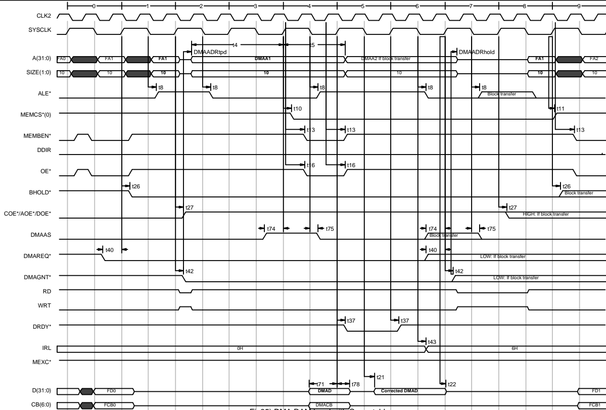
Fig35) DMA RAM Load with Correctable error
