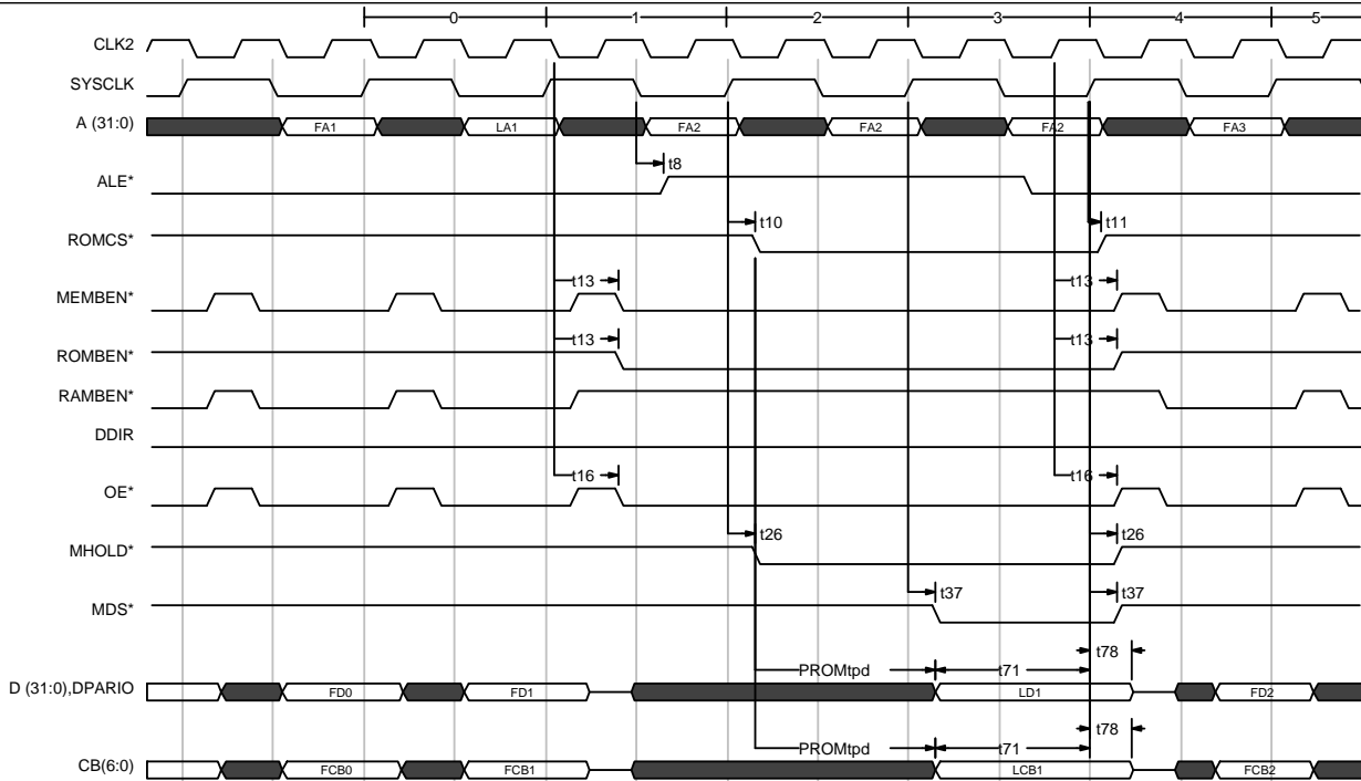
Fig 16) PROM 40 bit wide load at 2 WS
