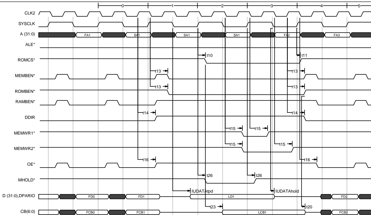
Fig 17) PROM 40 bit wide store at 1 WS
