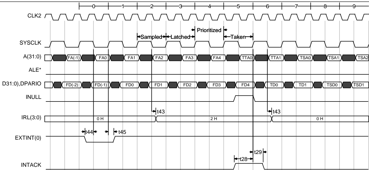
Fig 45) Edge triggered interrupt Timing
