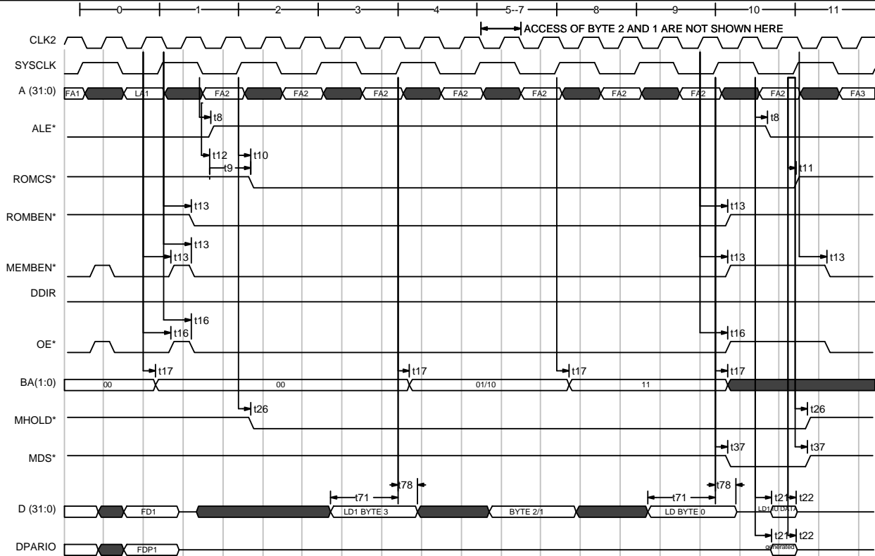
Figure 14) PROM bitwise Load at 2 waitstates
