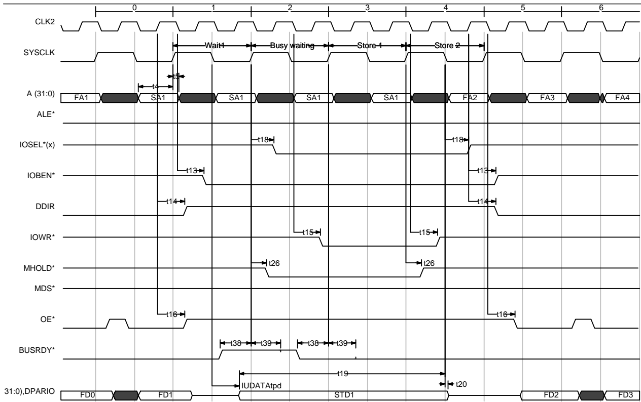
Fig 27) IO Store at 0 waitstates with Busy
