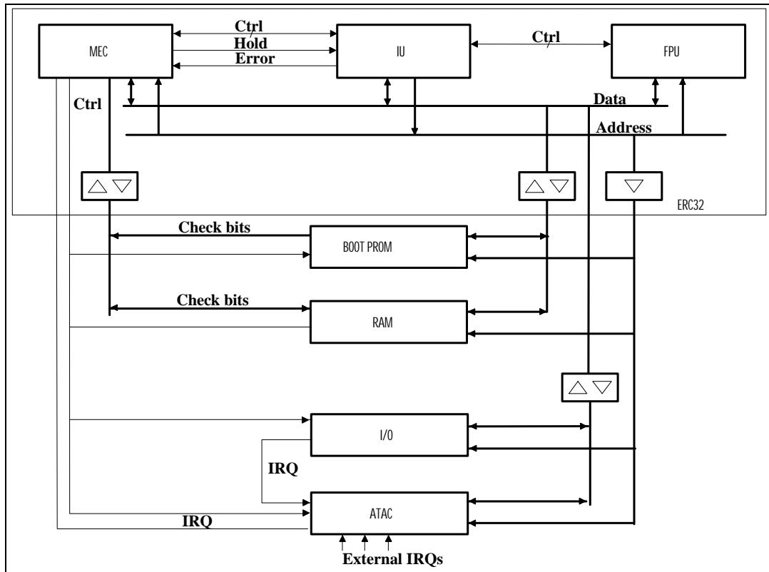
Figure 1 - ERC32 Computer with typical peripherals
