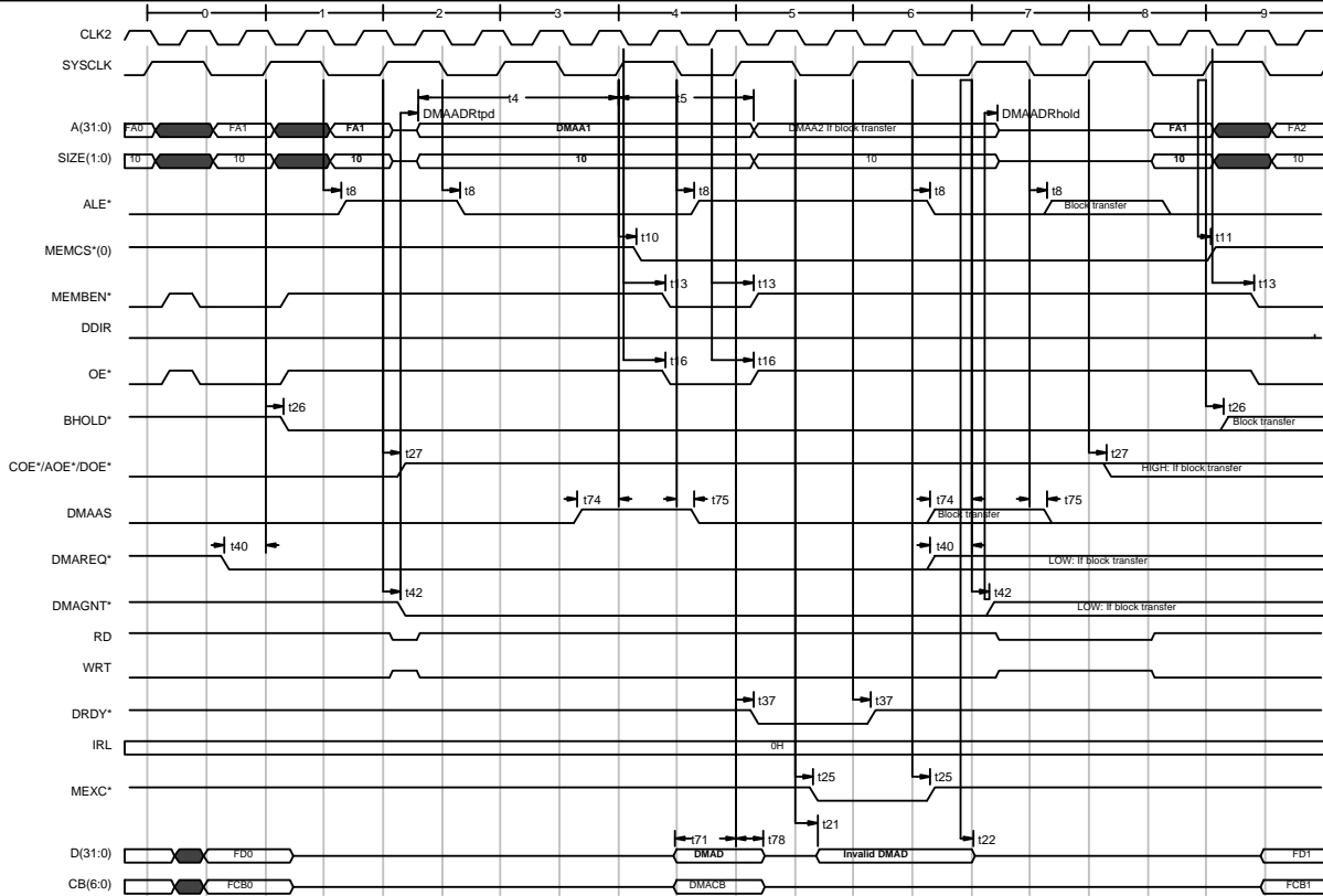
Fig36) DMA RAM Load with Uncorrectable error
