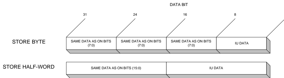
Figure 4 - Store Subword Data Layout
