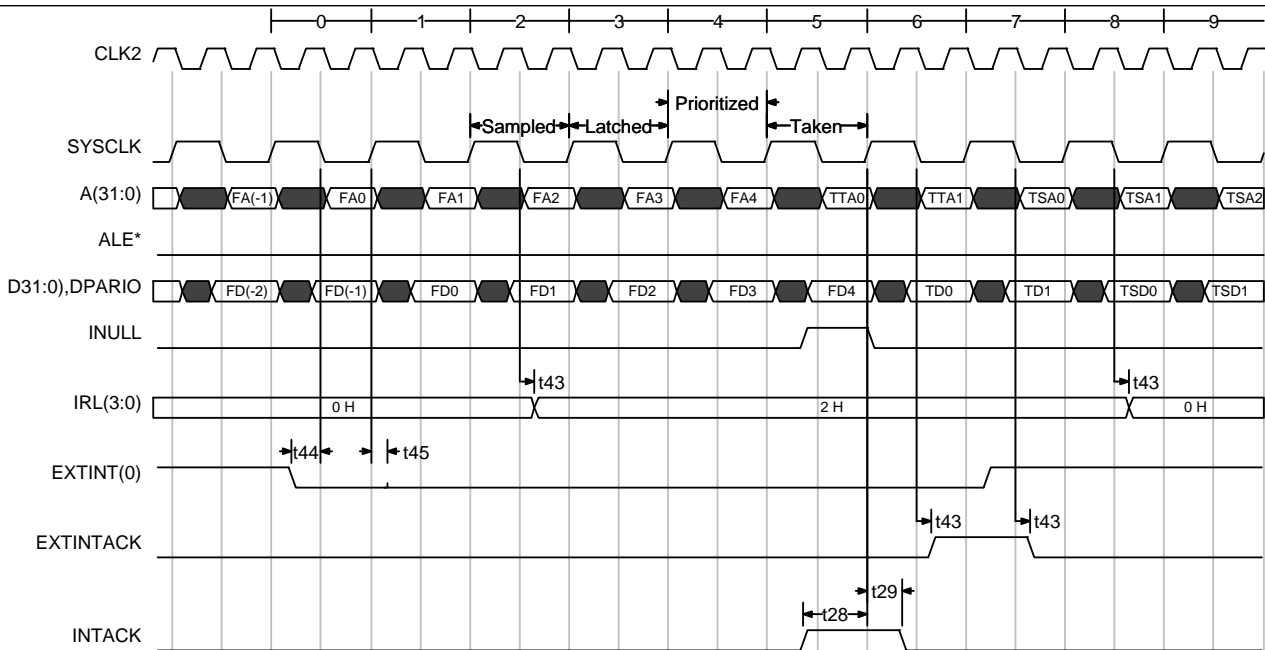
Fig 46) Level triggered interrupt Timing
