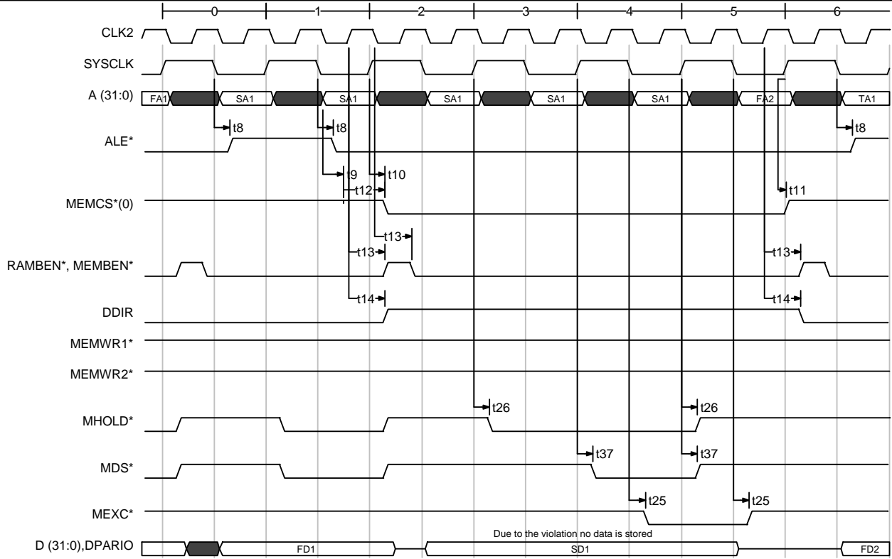
Figure 8) RAM Store at 1 waitstate with Access Violation
