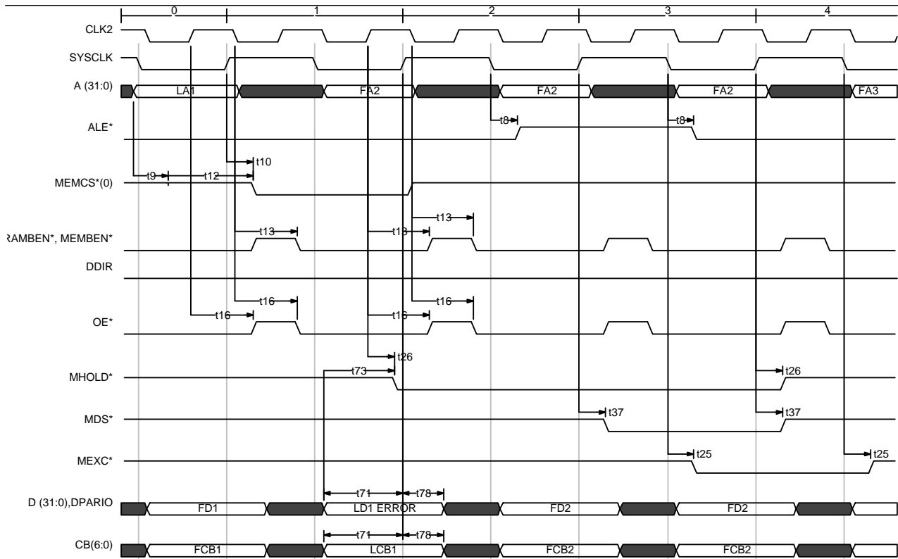
Figure 6) RAM Load with Uncorrectable Error at 0 WS
