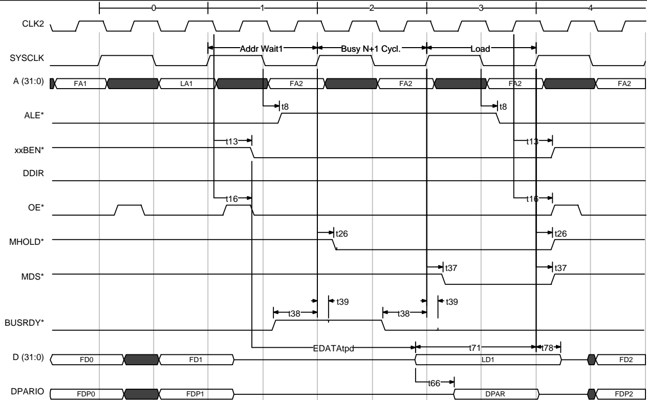
Fig 28) Extended Area Load with Busy
