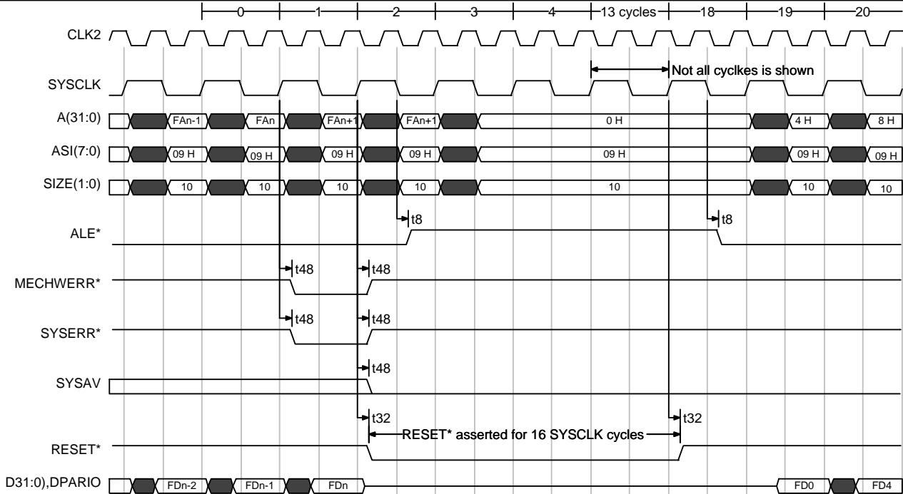
Fig 43) Internal MEC Error with Reset Timing
