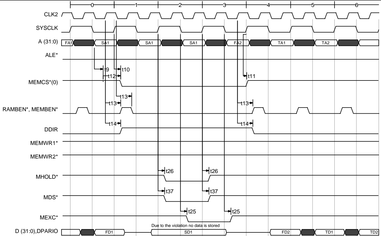
Figure 9) RAM Store at 0 waitstate with Access Violation
