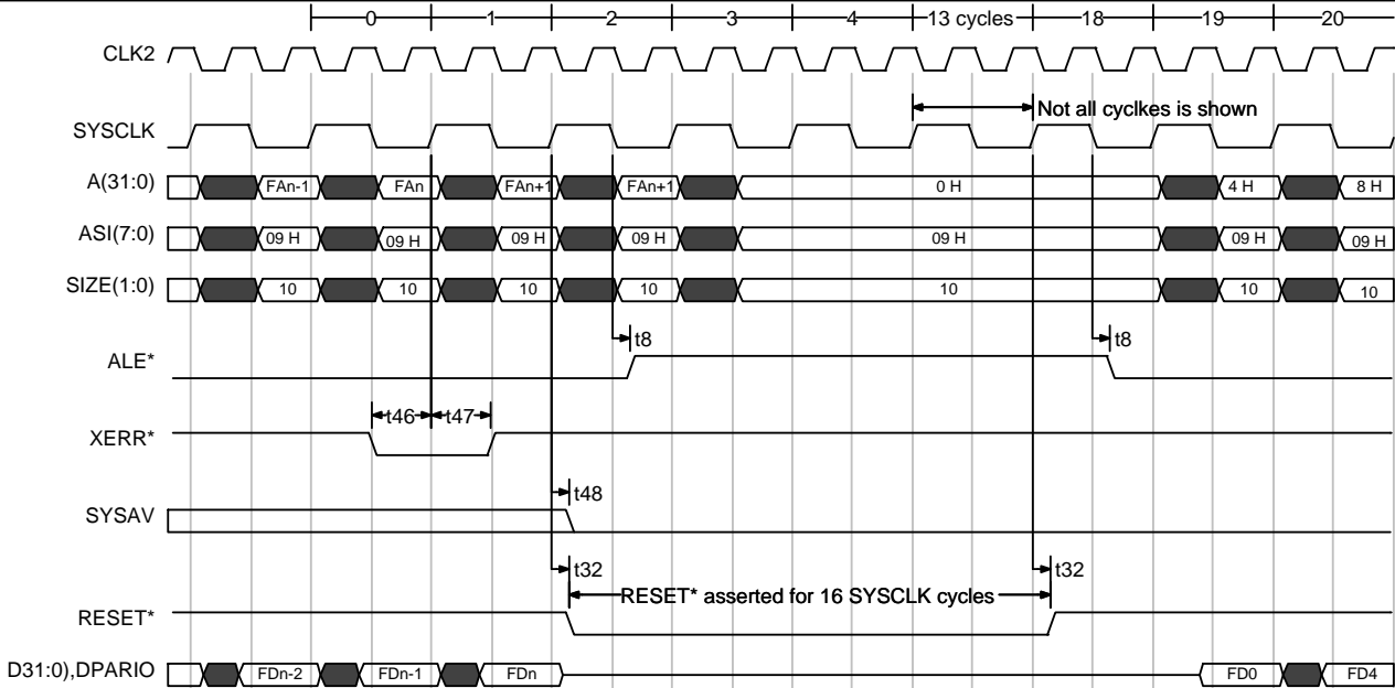
Fig 41) External Error with Reset Timing
