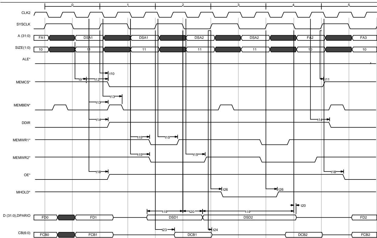
Figure 12) RAM Store Double at 0 WS
