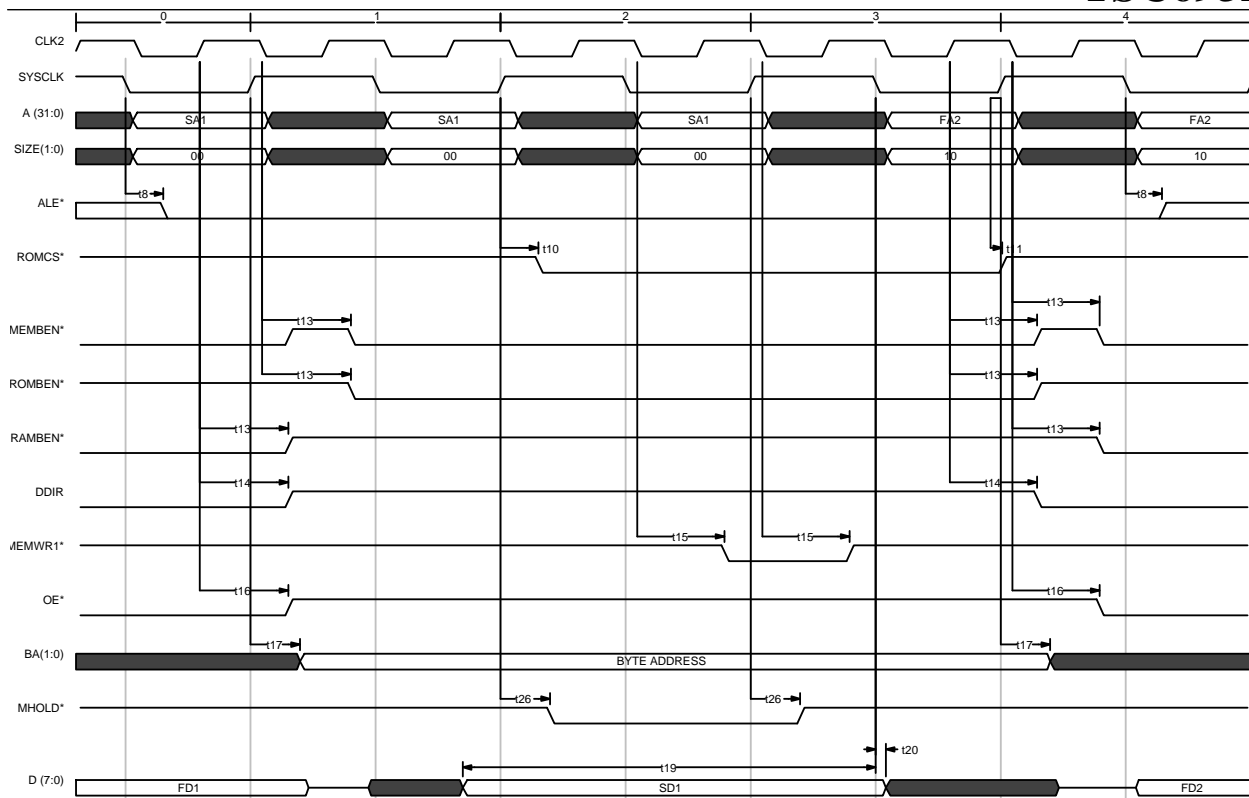
Fig 15) PROM Byte-wide Store at 1 WS
