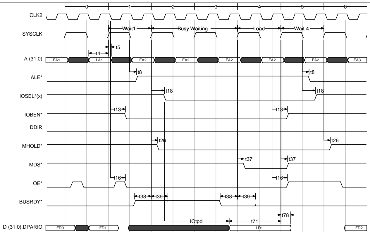
Fig 26) IO Load with Busy
