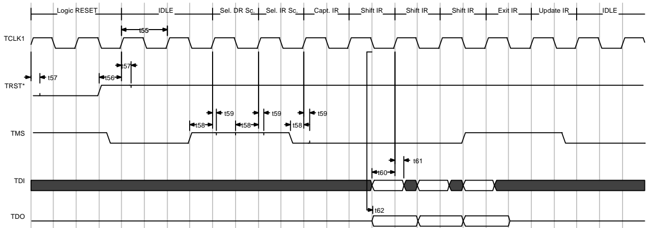
Fig 38) TAP Control Timing
