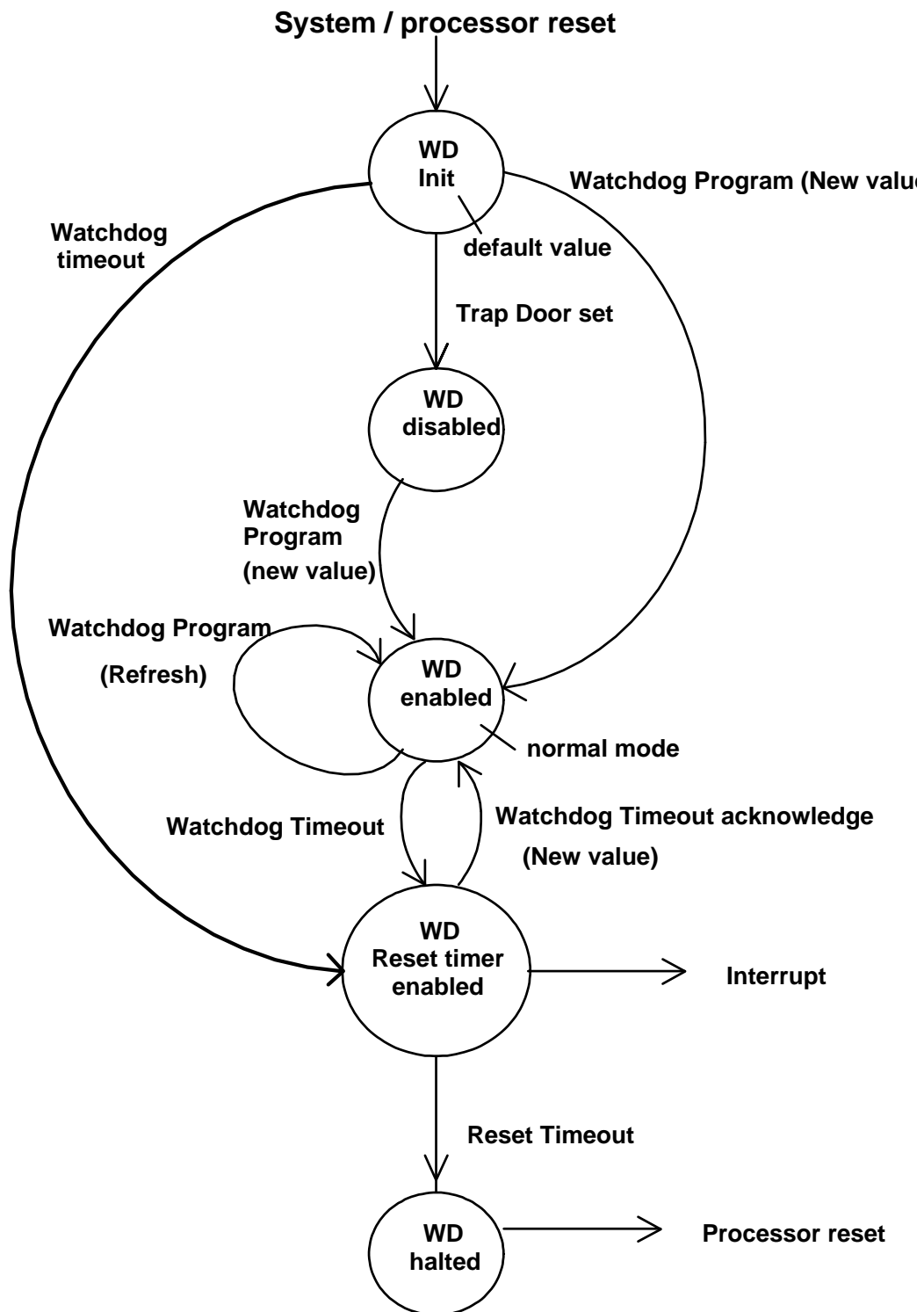
Figure 7 - Watchdog timer states and transitions
