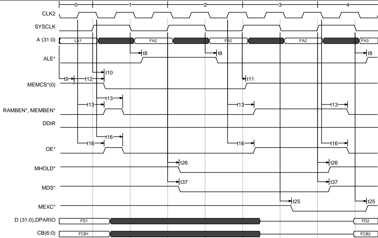
Figure 7) RAM Load at 1 Waitstate with Access Violation
