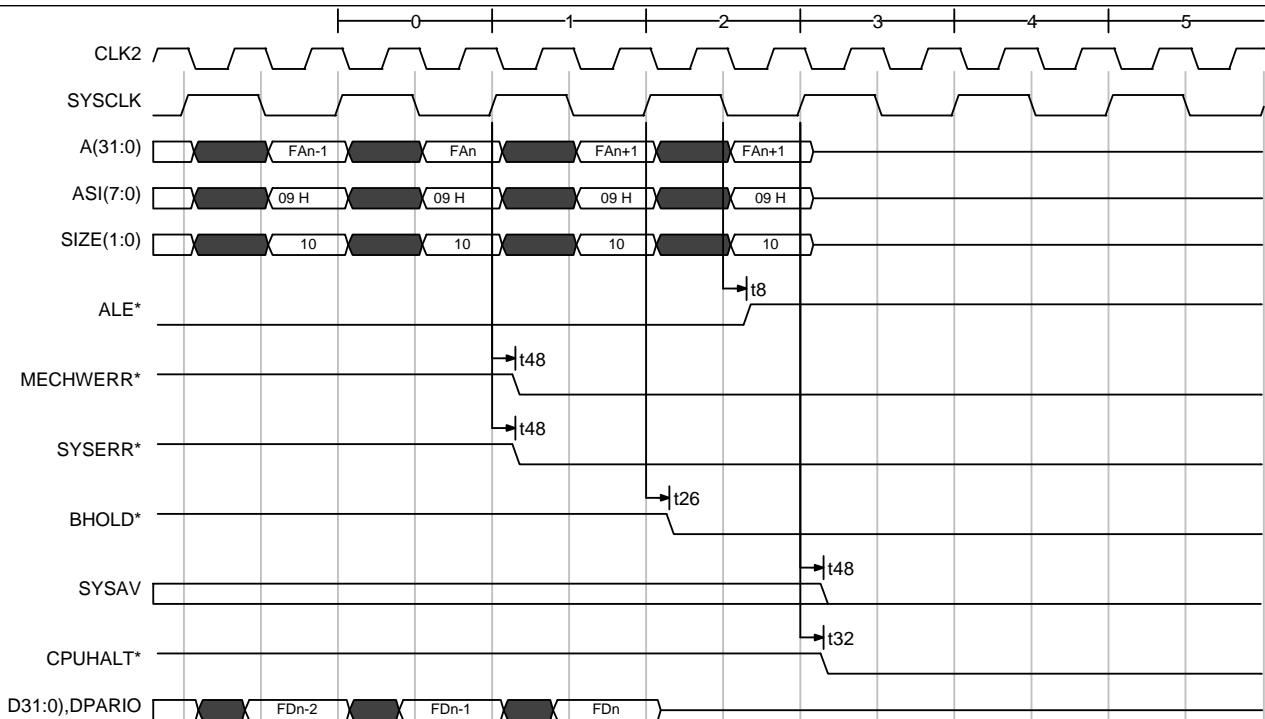
Fig 44) Internal MEC Error with Halt Timing
