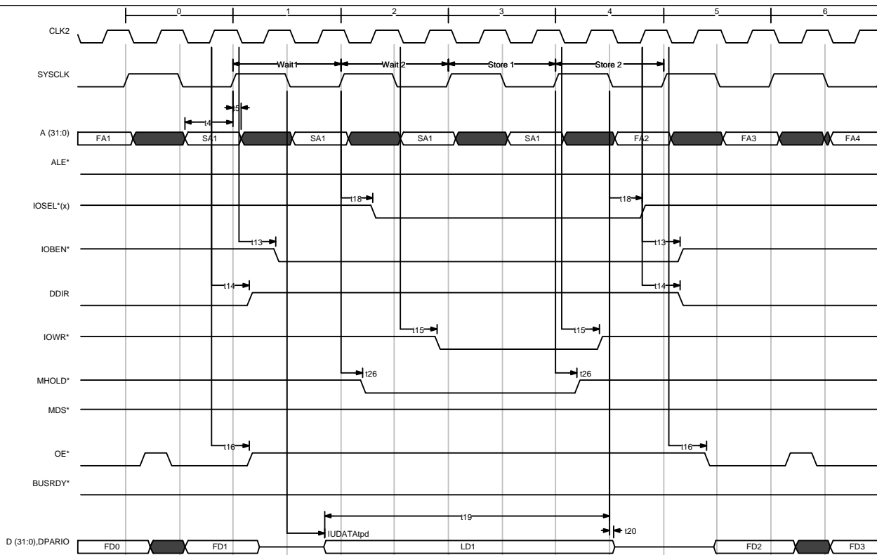
Fig 25) IO Store at 2 waitstates
