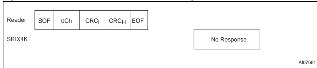
Figure 61. READ_BLOCK frame exchange between Reader and SRIX4K
