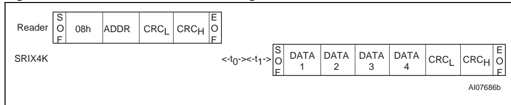
Figure 62. WRITE_BLOCK frame exchange between Reader and SRIX4K
