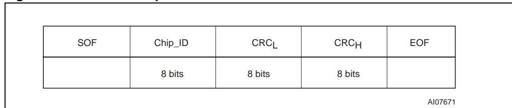
Figure 27. PCALL16 response format
