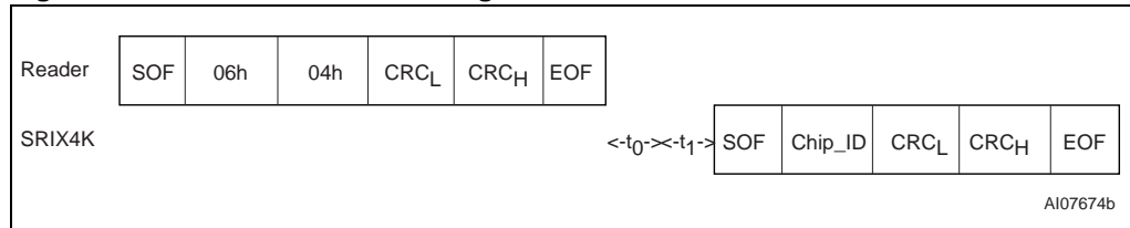
Figure 57. SLOT_MARKER frame exchange between Reader and SRIX4K
