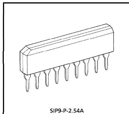
SIP9-P-2.54A Weight : 0.92g (Typ.)
