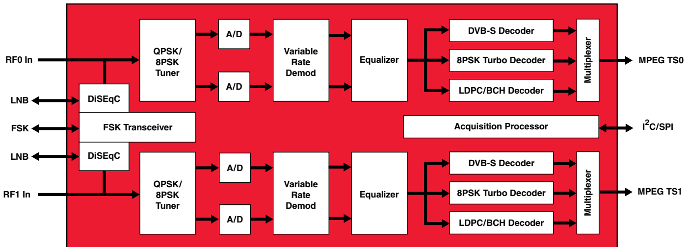
BCM4506 Block Diagram
