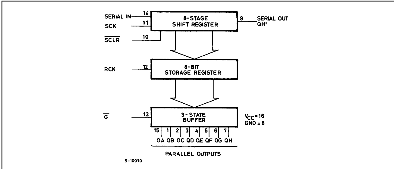
Figure 3: Logic Diagram
