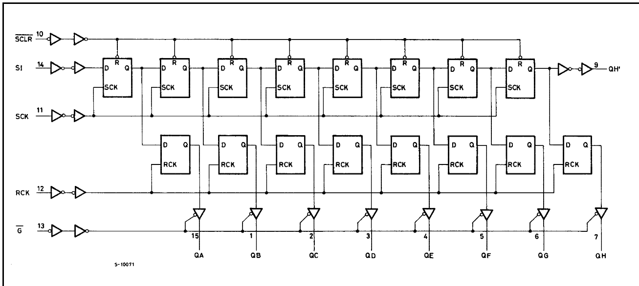
Figure 4: Logic Diagram
