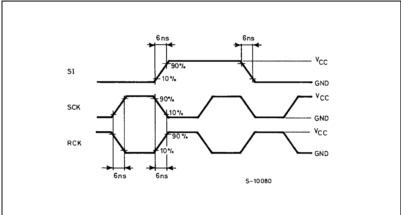
Figure 14: Waveform - Input Waveform (f=1MHz; 50% duty cycle)
