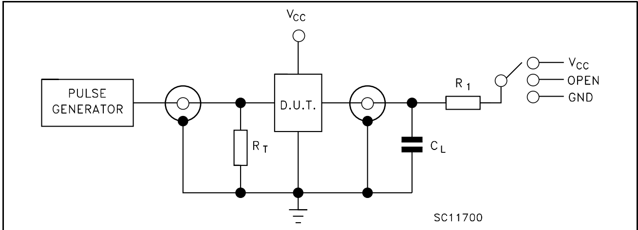
Figure 7: Test Circuit
