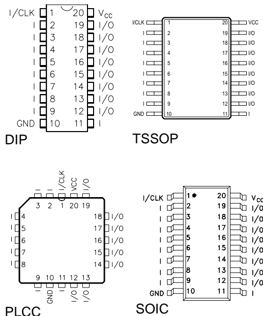
Figure 1 Pin Configuration
