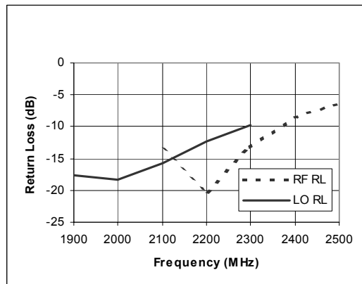
Figure 9. RF and LO Return Loss versus Frequency
