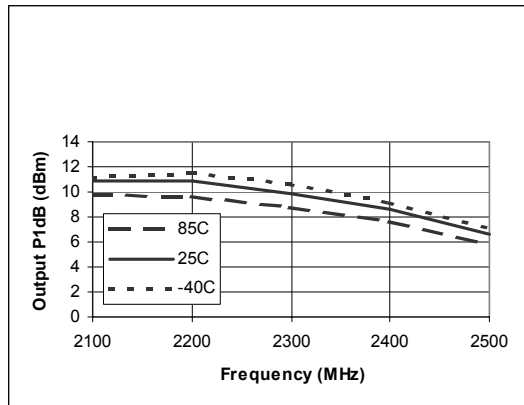
Figure 10. Output P1dB versus Frequency + Temperature
