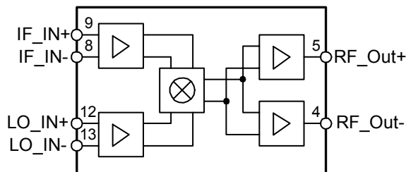
Figure 1. Block Diagram
