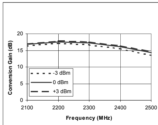
Figure 5. Conversion Gain versus Frequency + LO Drive
