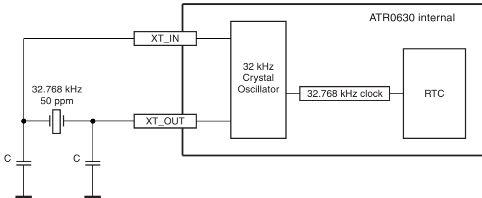
Figure 5-5. Crystal Connection
