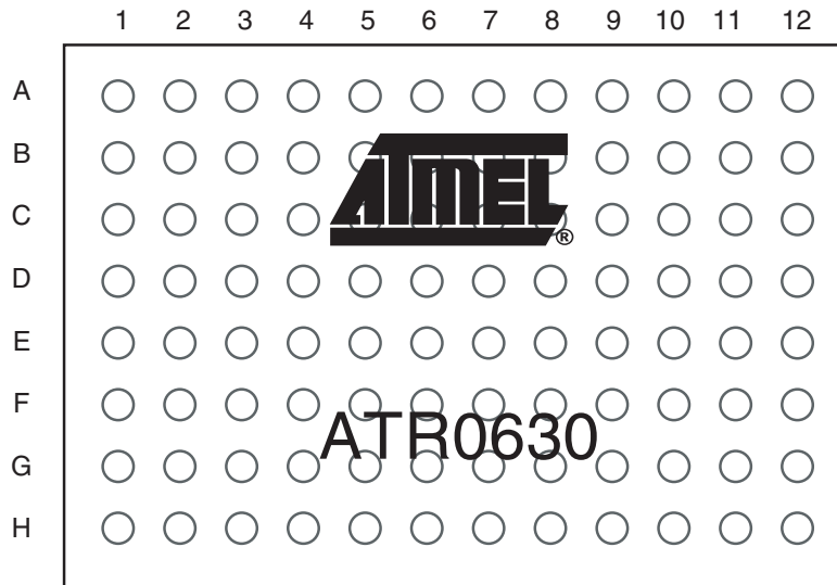
Figure 3-1. Pinning BGA96 (Top View)
