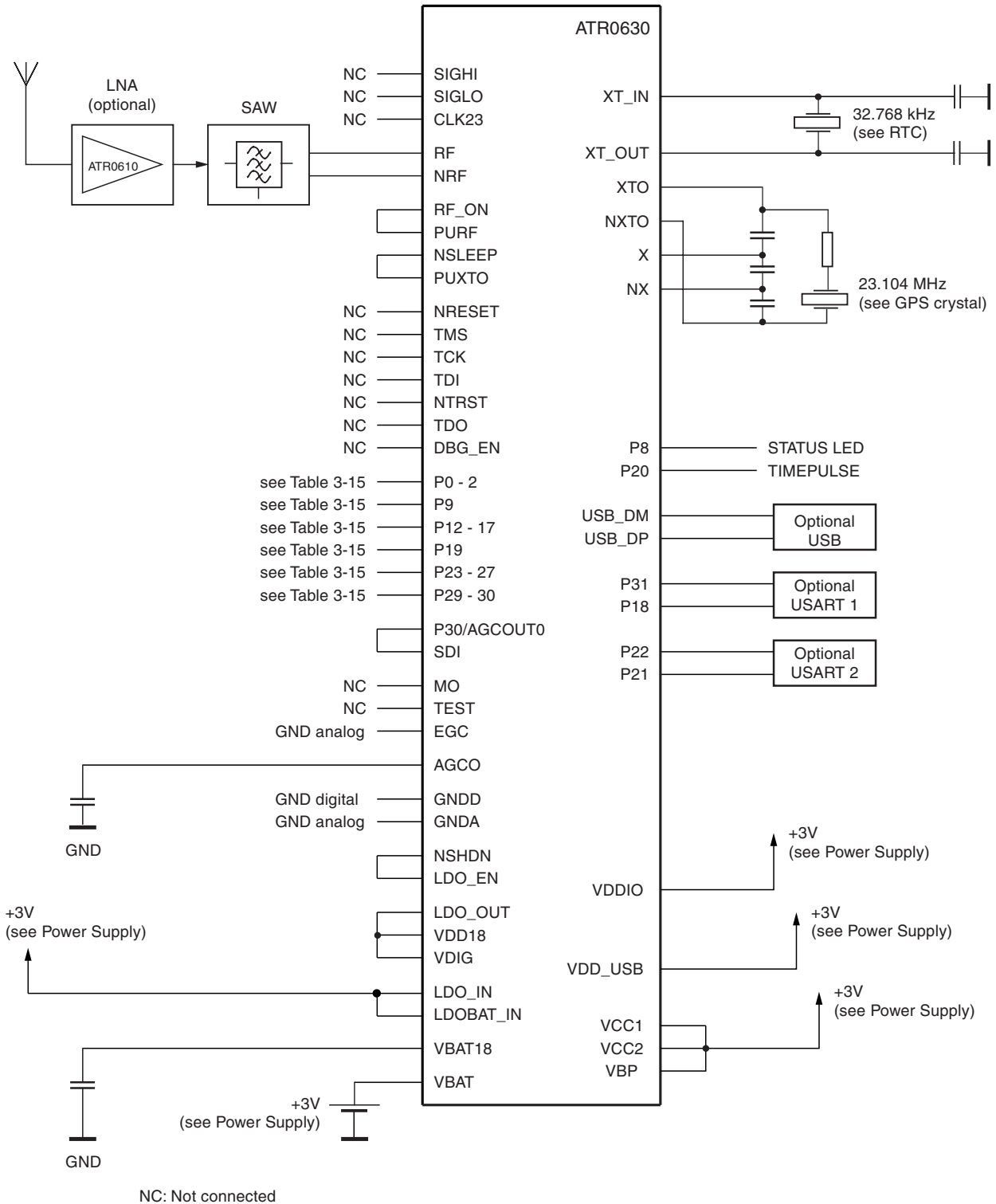
Figure 3-2. Example of an External Connection (ATR0630)
