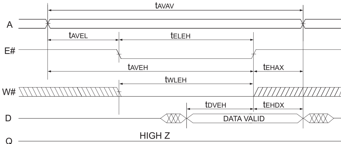
FIG. 4 WRITE CYCLE — E# CONTROLLED
