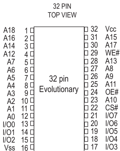
FIGURE 1 – PIN CONFIGURATION
