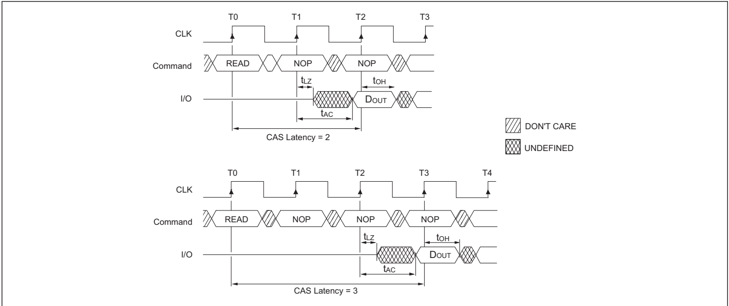
FIGURE 4 – CAS LATENCY
