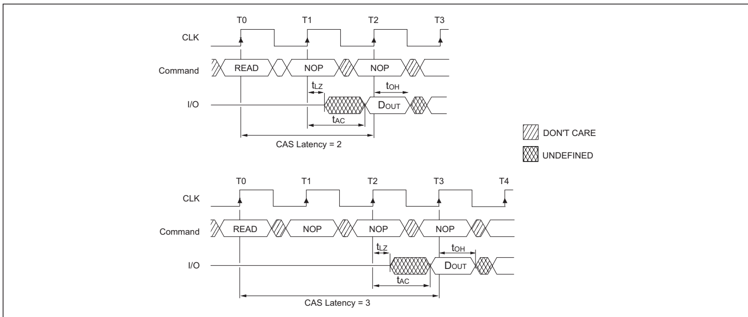
FIGURE. 4 – CAS LATENCY
