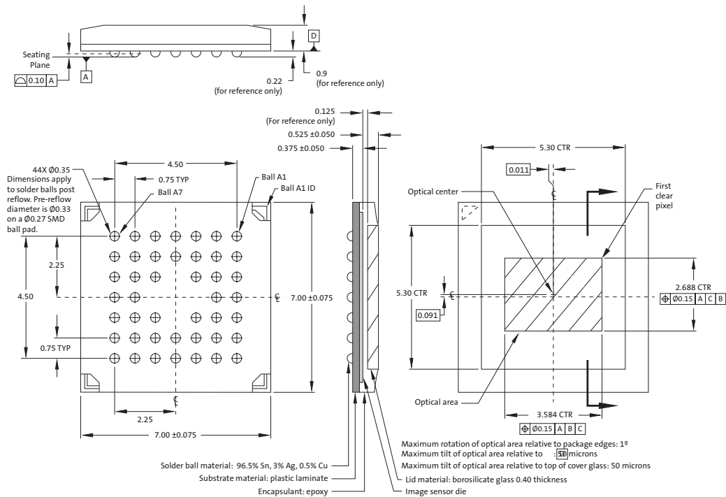
Figure 1: 44-Ball ICSP Package (Pb-Free) Outline Drawing
