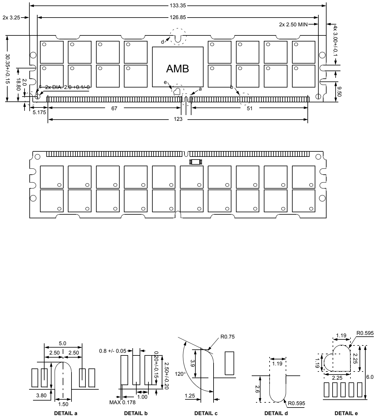
Figure 18 : FBDIMM Physical Dimension -1 (For PCB) : 256Mbx4 based 512Mx72 Module (2Rank) M395T5160CZ4
