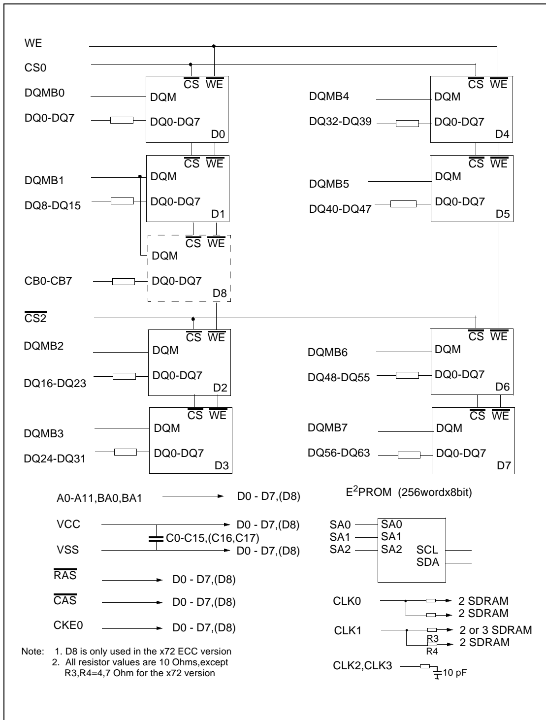
Block Diagram for 8M x 64/72 SDRAM DIMM modules
