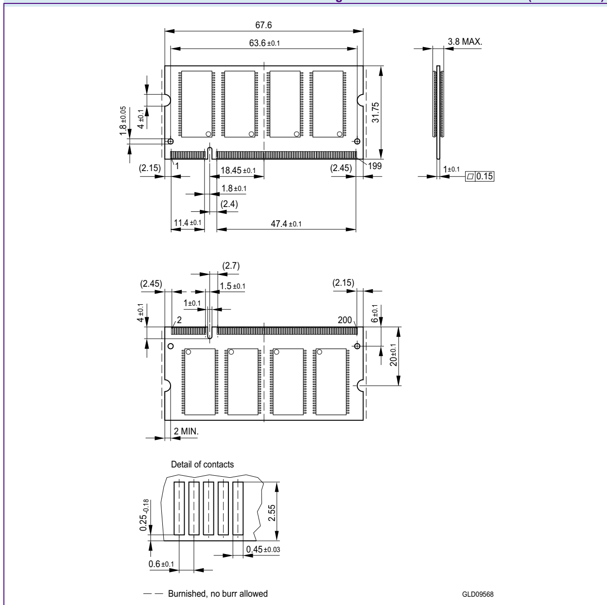
FIGURE 2 Package Outline SO-DIMM Raw Card A (L-DIM-200-6)
