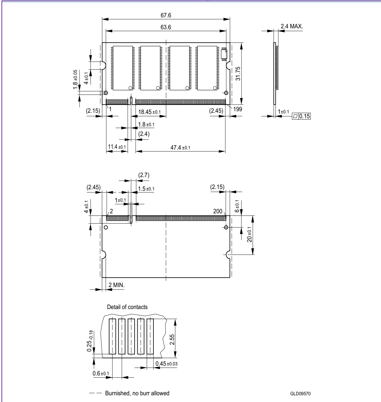
Package Outline SO-DIMM Raw Card C (L-DIM-200-11)
