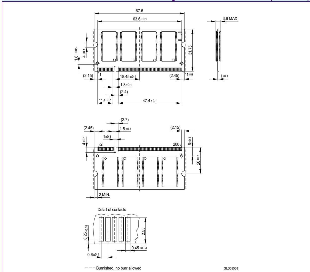
FIGURE 2 Package Outline SO-DIMM Raw Card A (L-DIM-200-6)
