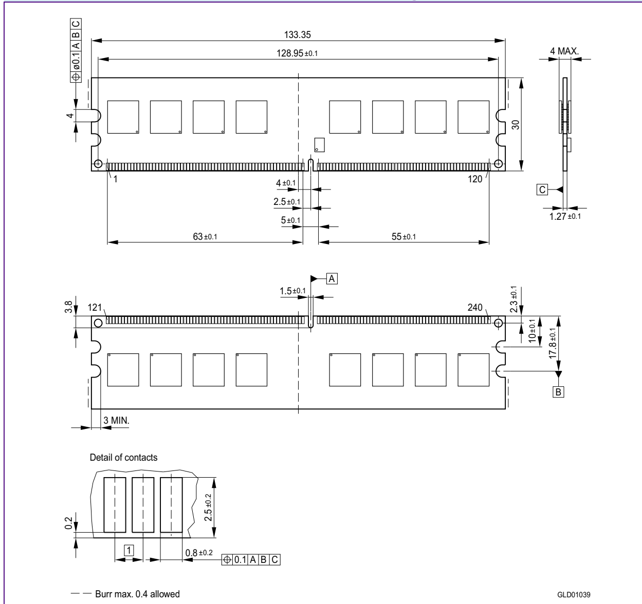
FIGURE 7 Package Outline L-DIM-240-109 Raw Card E
