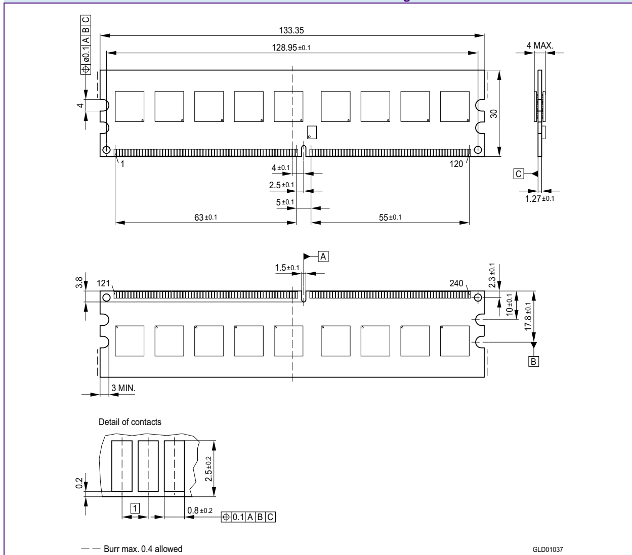
FIGURE 6 Package Outline L-DIM-240-107 Raw Card G
