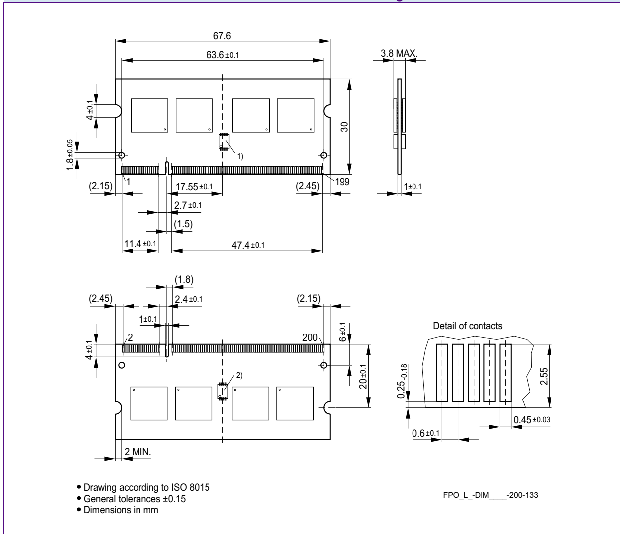
FIGURE 5 Package Outline L-DIM-200-133 Raw Card D
