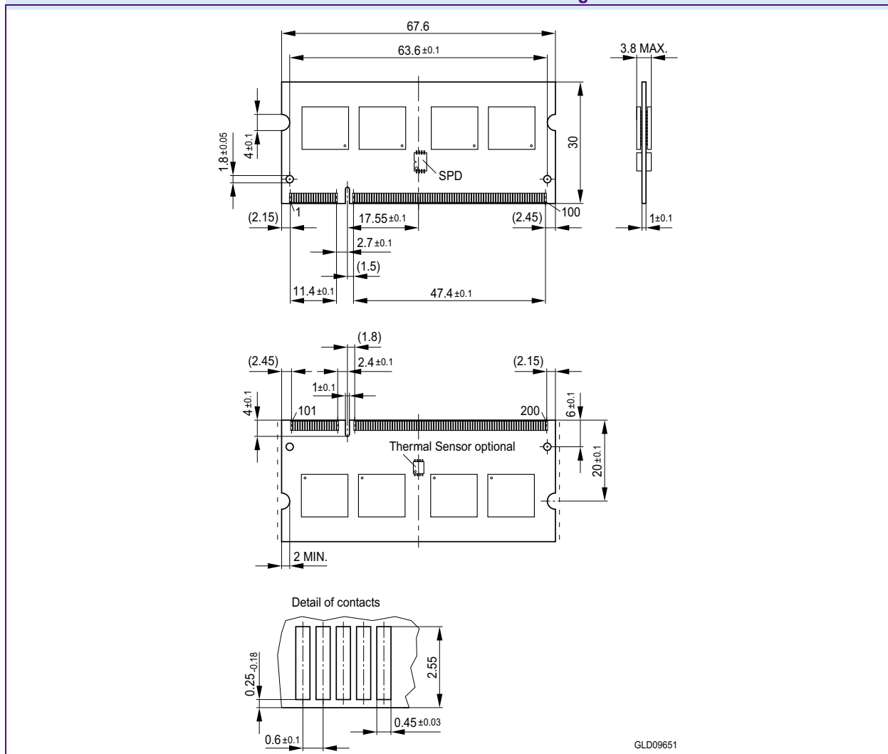
FIGURE 5 Package Outline Raw Card D L-DIM-200-33
