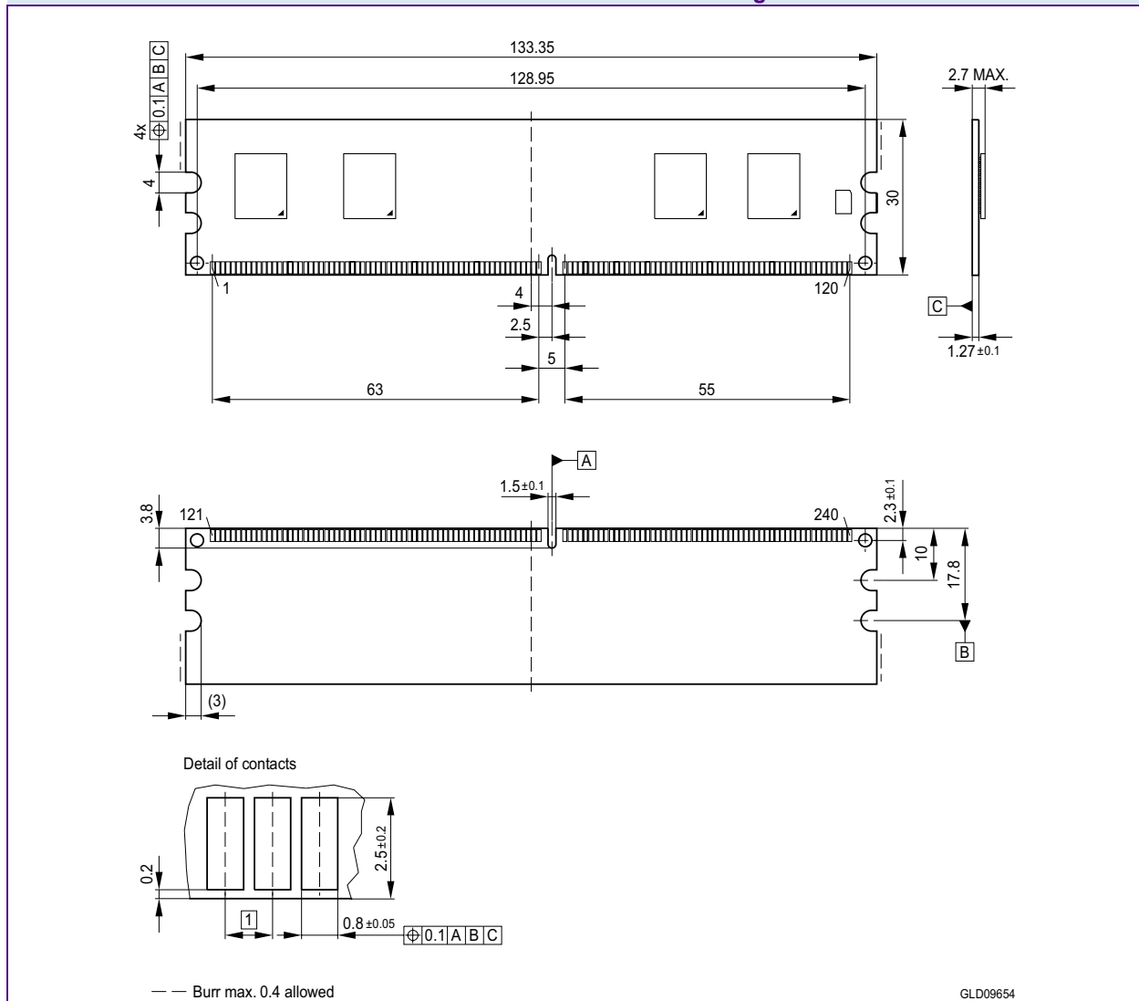
FIGURE 6 Package Outline L-DIM-240-3 Raw Card C
