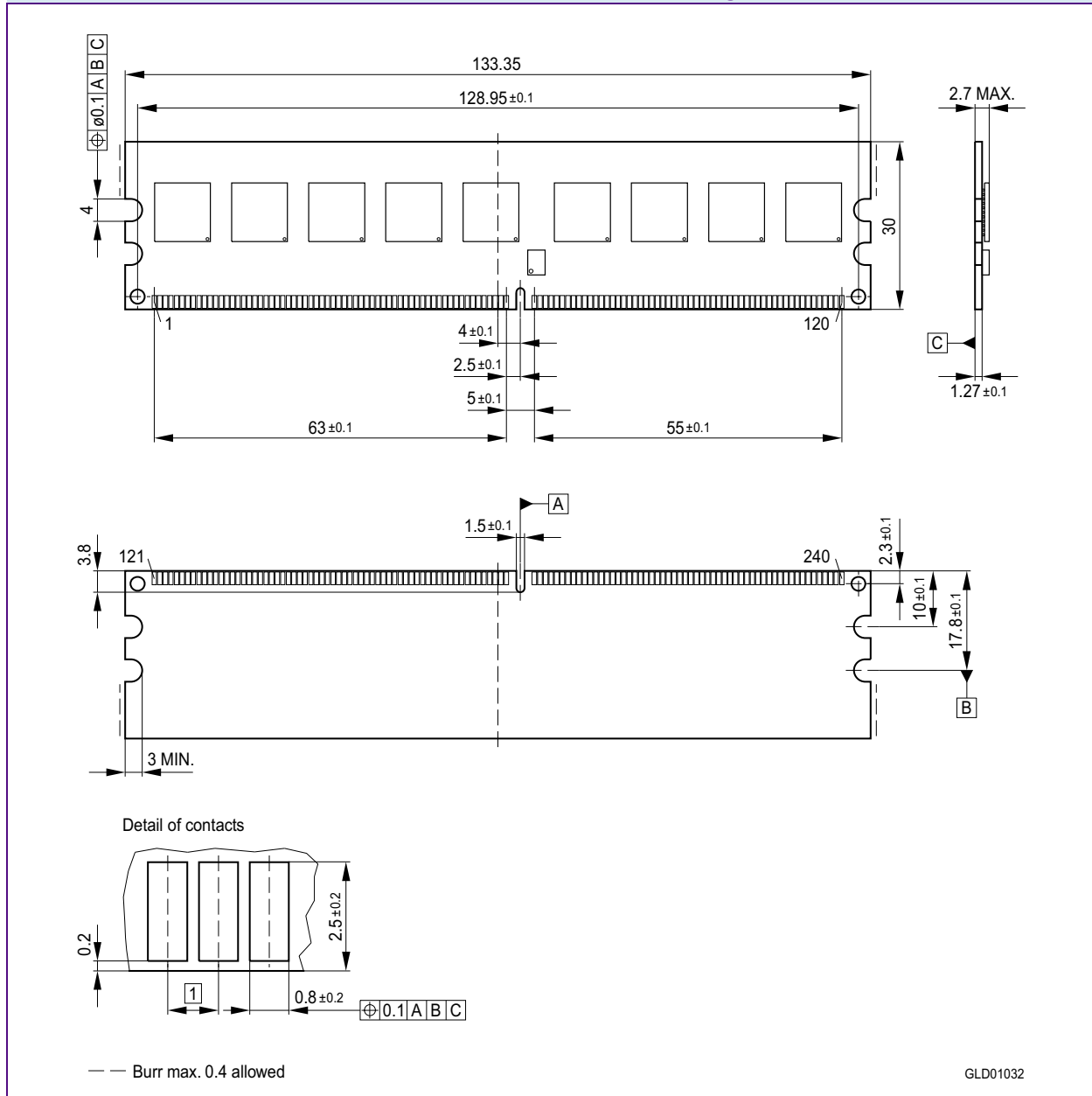
FIGURE 7 Package Outline L-DIM-240-6 Raw Card F
