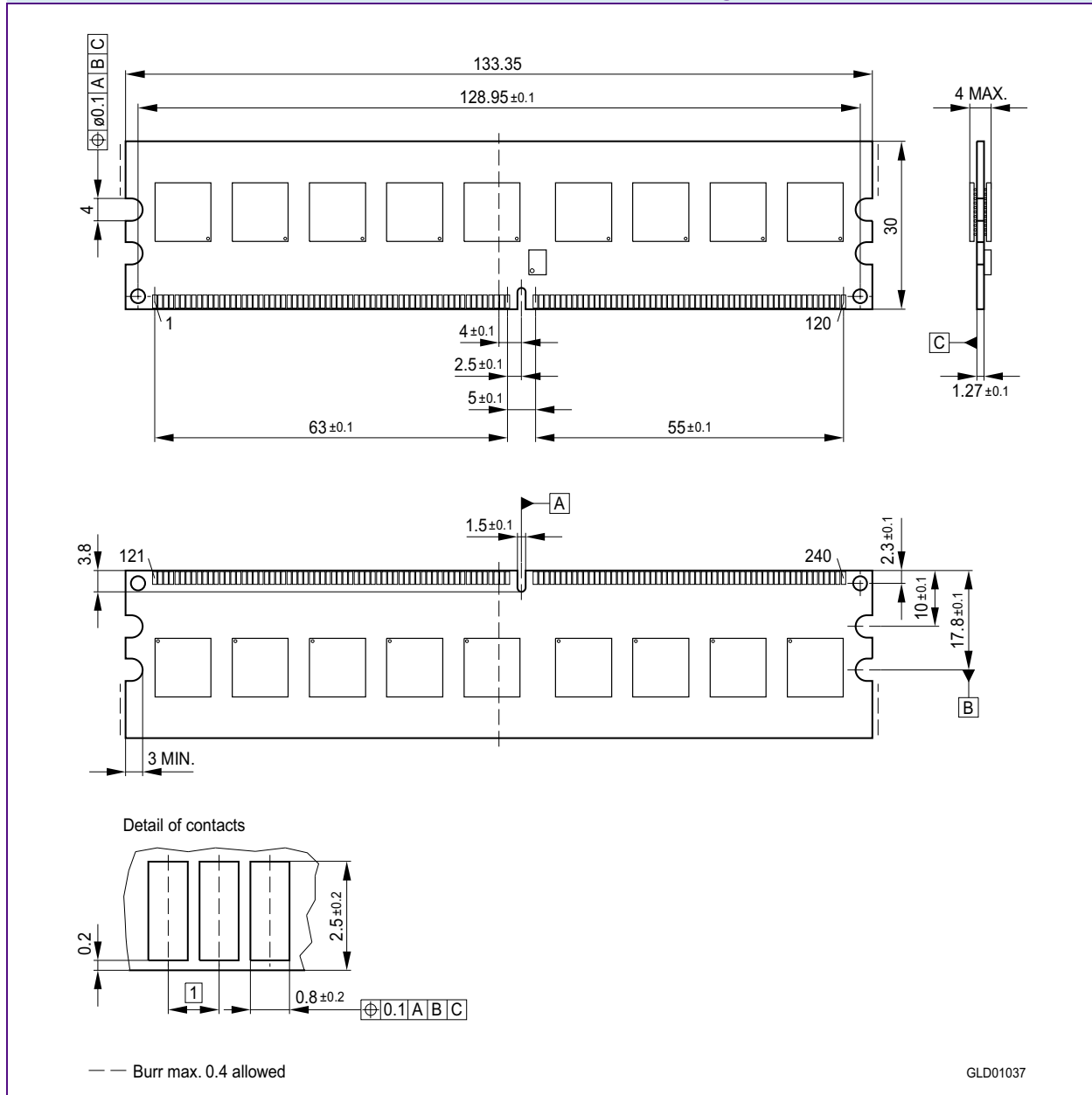
FIGURE 8 Package Outline L-DIM-240-7 Raw Card G
