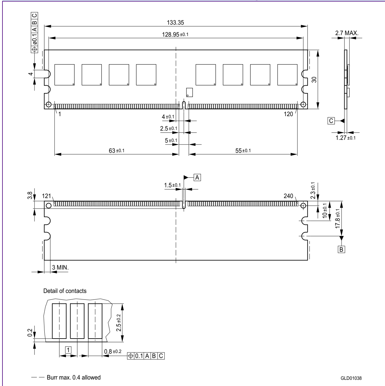
FIGURE 9 Package Outline L-DIM-240-8 Raw Card D
