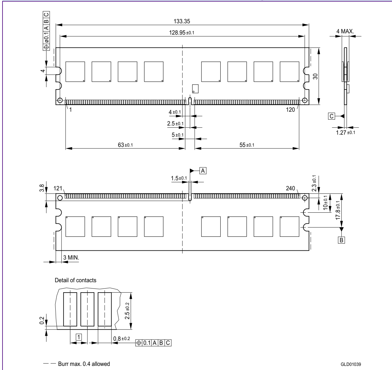
FIGURE 10 Package Outline L-DIM-240-9 Raw Card E
