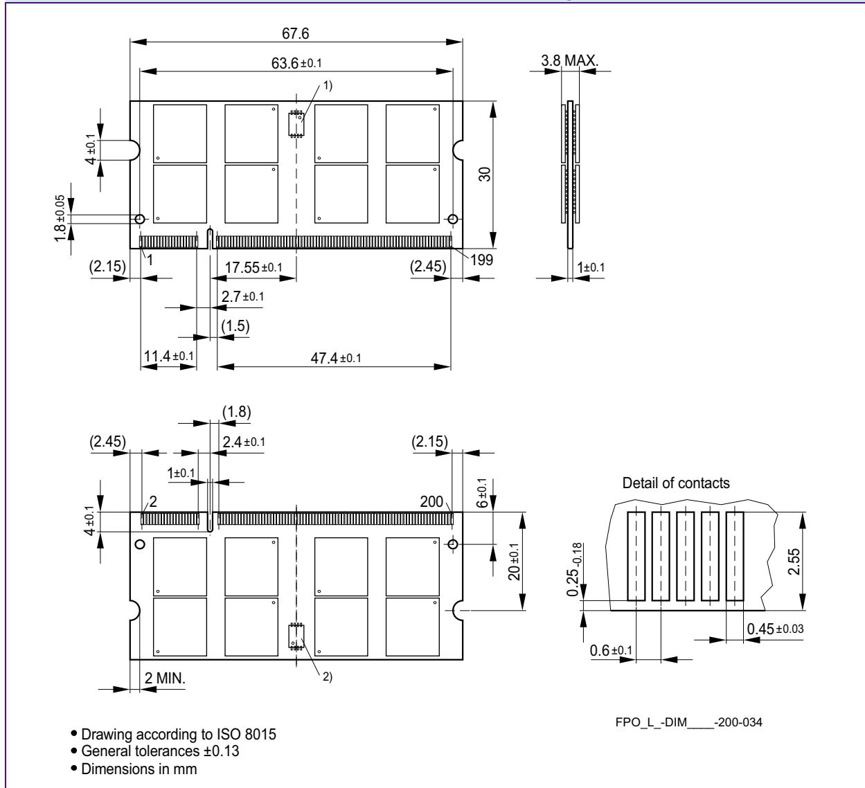
FIGURE 6 Package Outline L-DIM-200-34 Raw Card F
