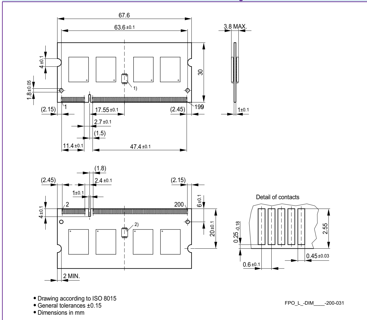
FIGURE 5 Package Outline L-DIM-200-31 Raw Card A
