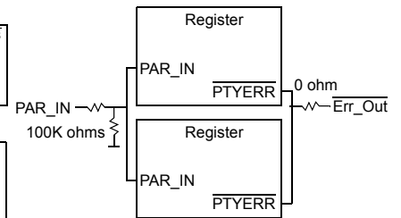
Signals for Address and Command Parity Function (M393T1K66AZA)
