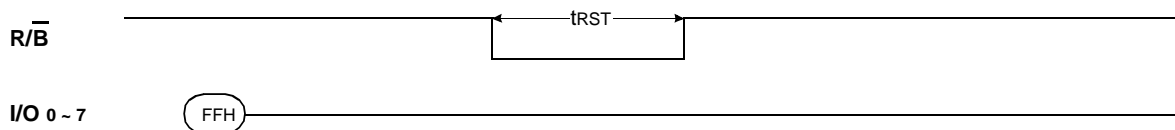
Figure 10. RESET Operation
