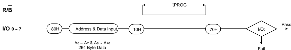
Figure 7. Program &amp; Read Status Operation
