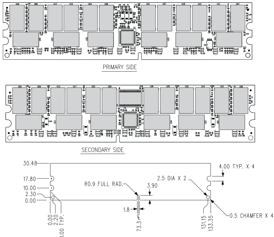
Figure 1: KVR333X72BRC25/1G 184-Pin DIMM
