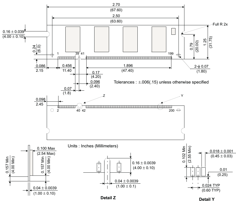
Figure 1: KVR333X64SC25/128 200-Pin SODIMM
