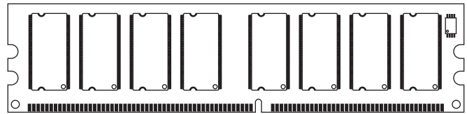
Figure 3: Reduced-Height Layout
