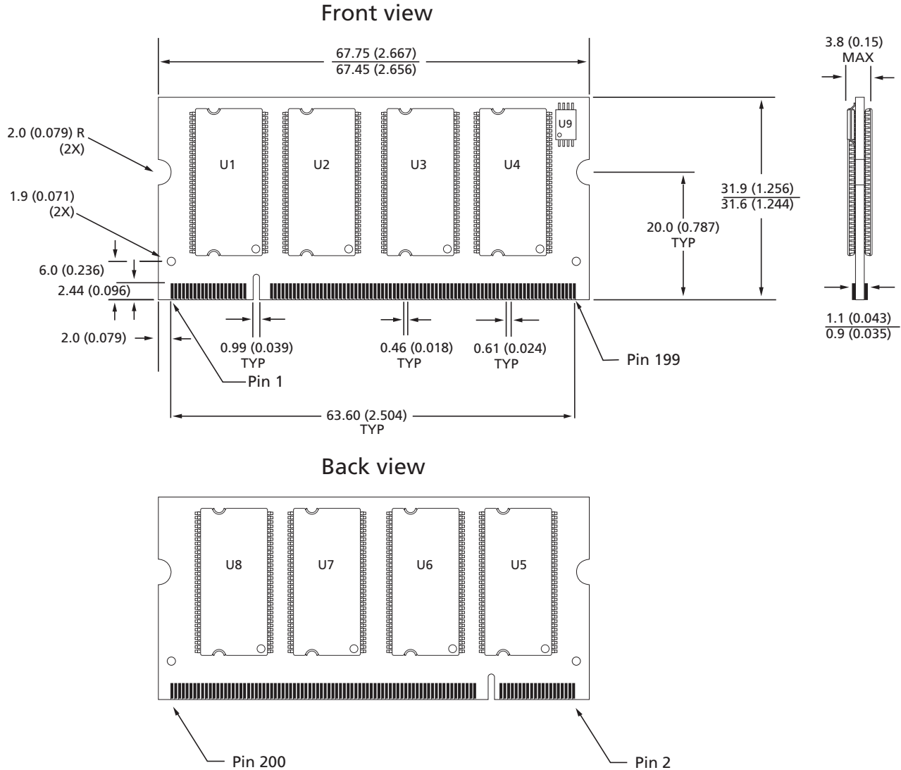
Figure 4: 200-Pin SODIMM – Layout 1 (128MB, 256MB)
