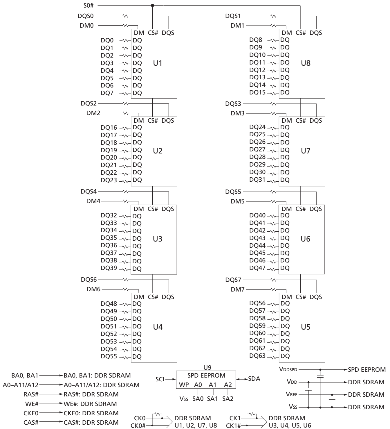
Figure 3: Functional Block Diagram – Layout 2 (128MB, 256MB, 512MB)
