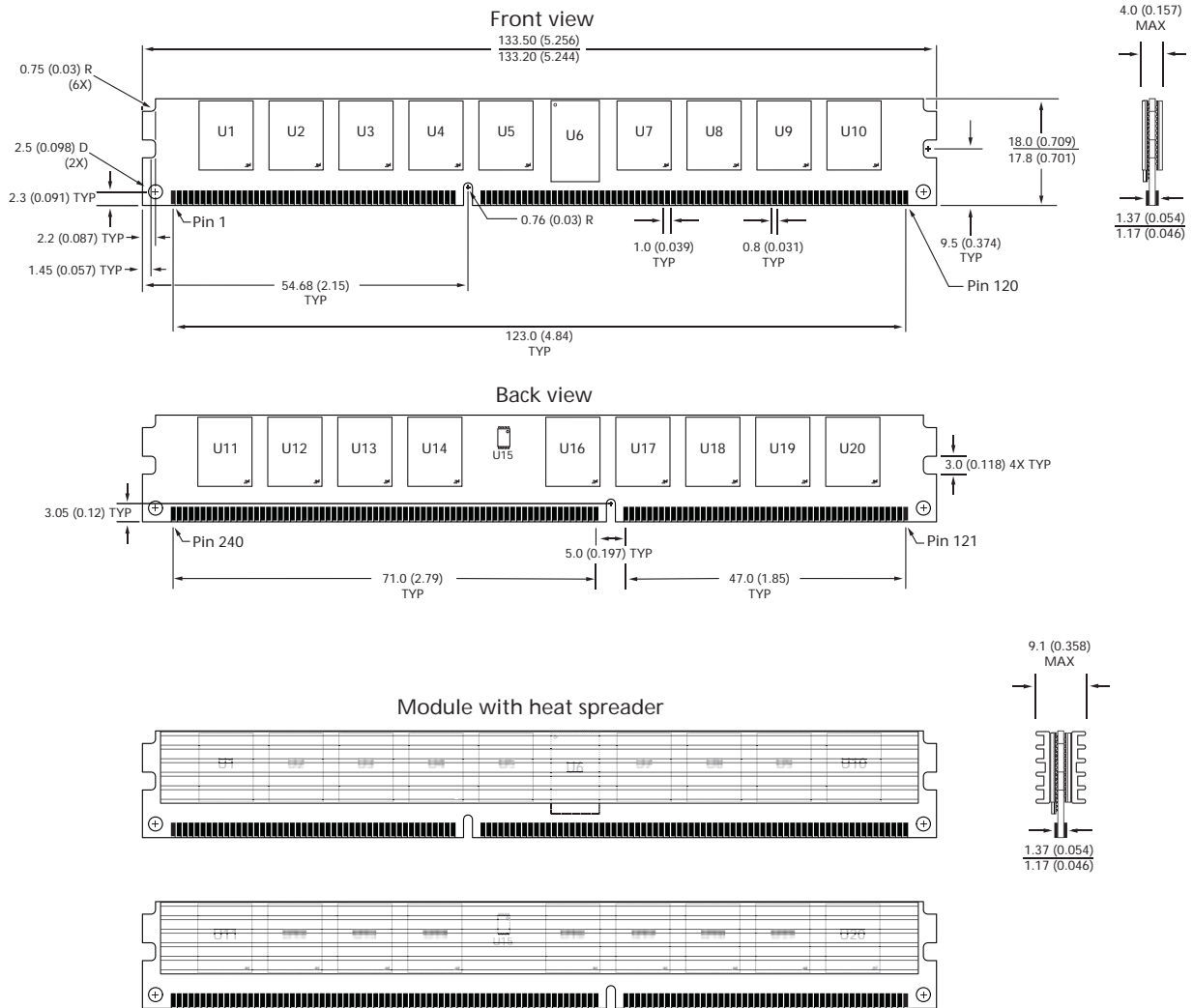
Figure 5: 240-Pin DDR3 VLP RDIMM
