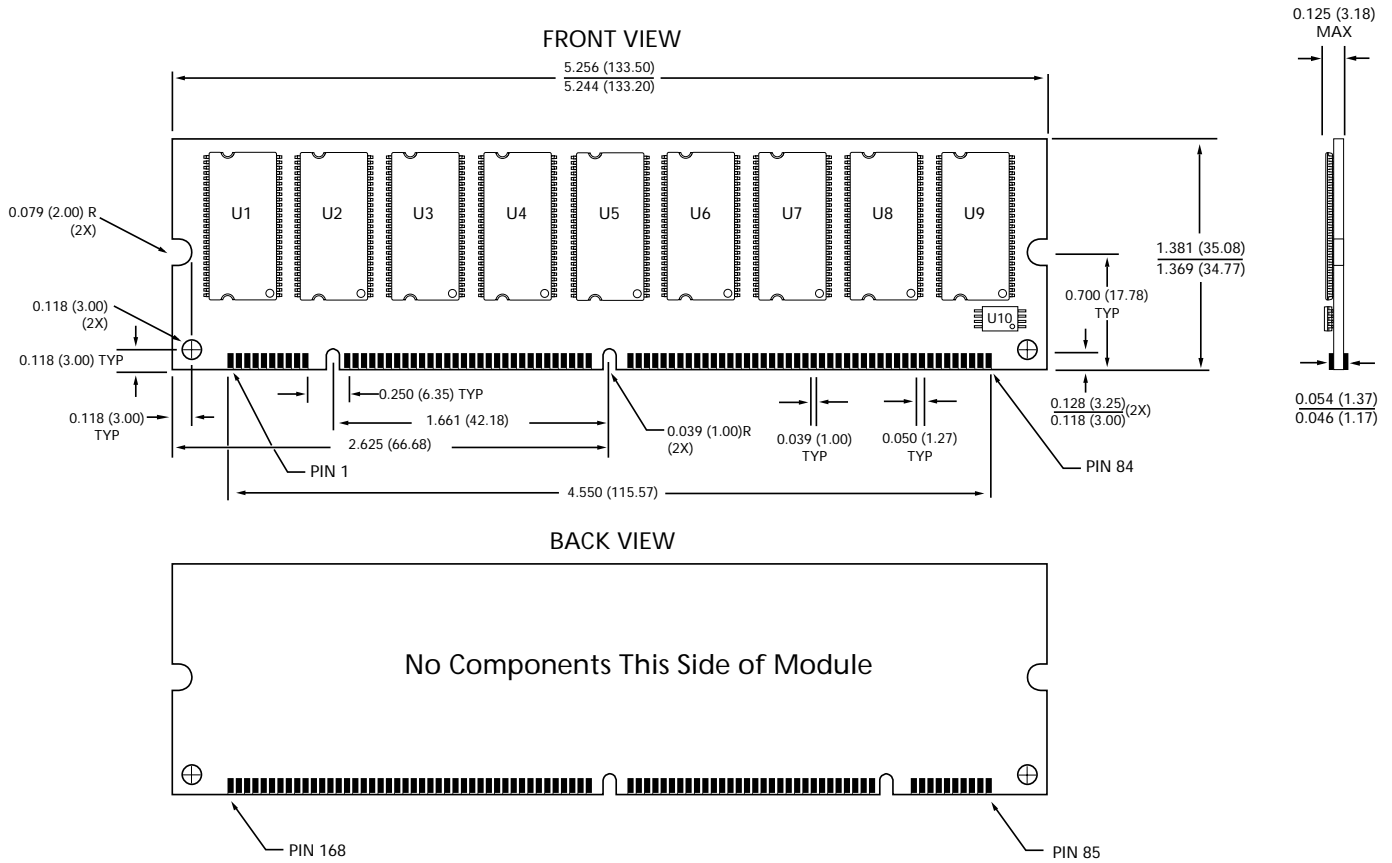
Figure 11: 168-Pin DIMM Dimensions – Single-Rank
