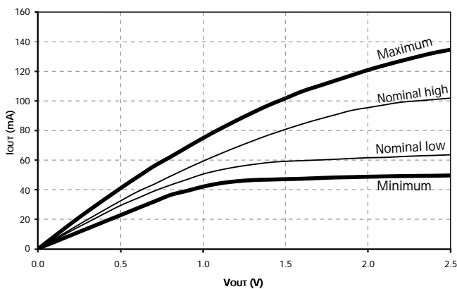
Figure 8: Pull-Down Characteristics
