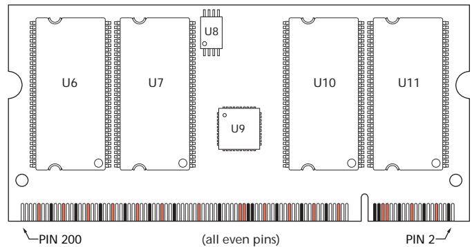
Figure 2: Module Layout
