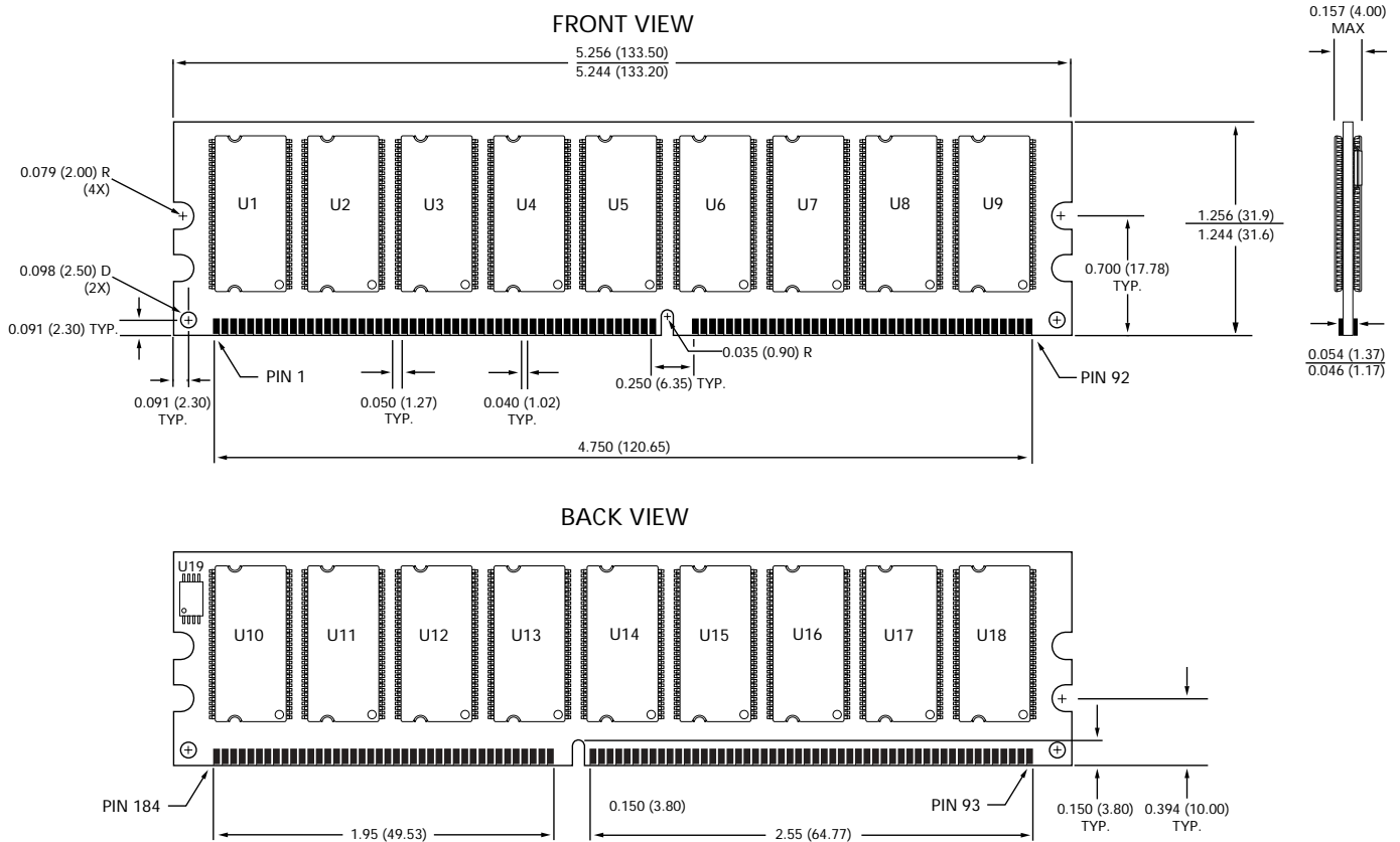
Figure 16: 184-PIN DIMM Dimensions
