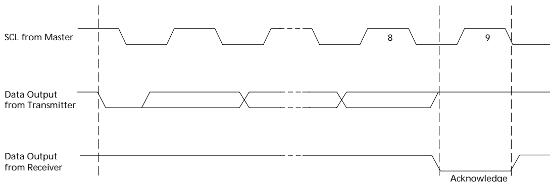
Figure 14: Acknowledge Response From Receiver
