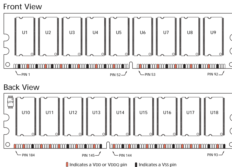
Figure 2: Pin Locations: 184-Pin DIMM
