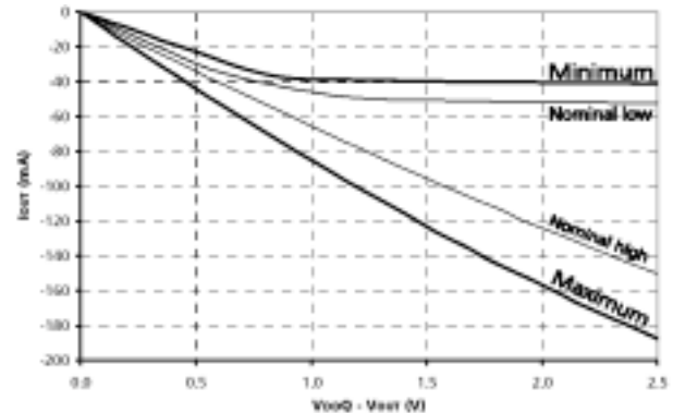
Figure 9: Pull-Up Characteristics
