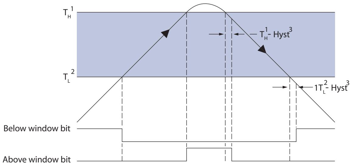
Figure 4: Hysteresis
