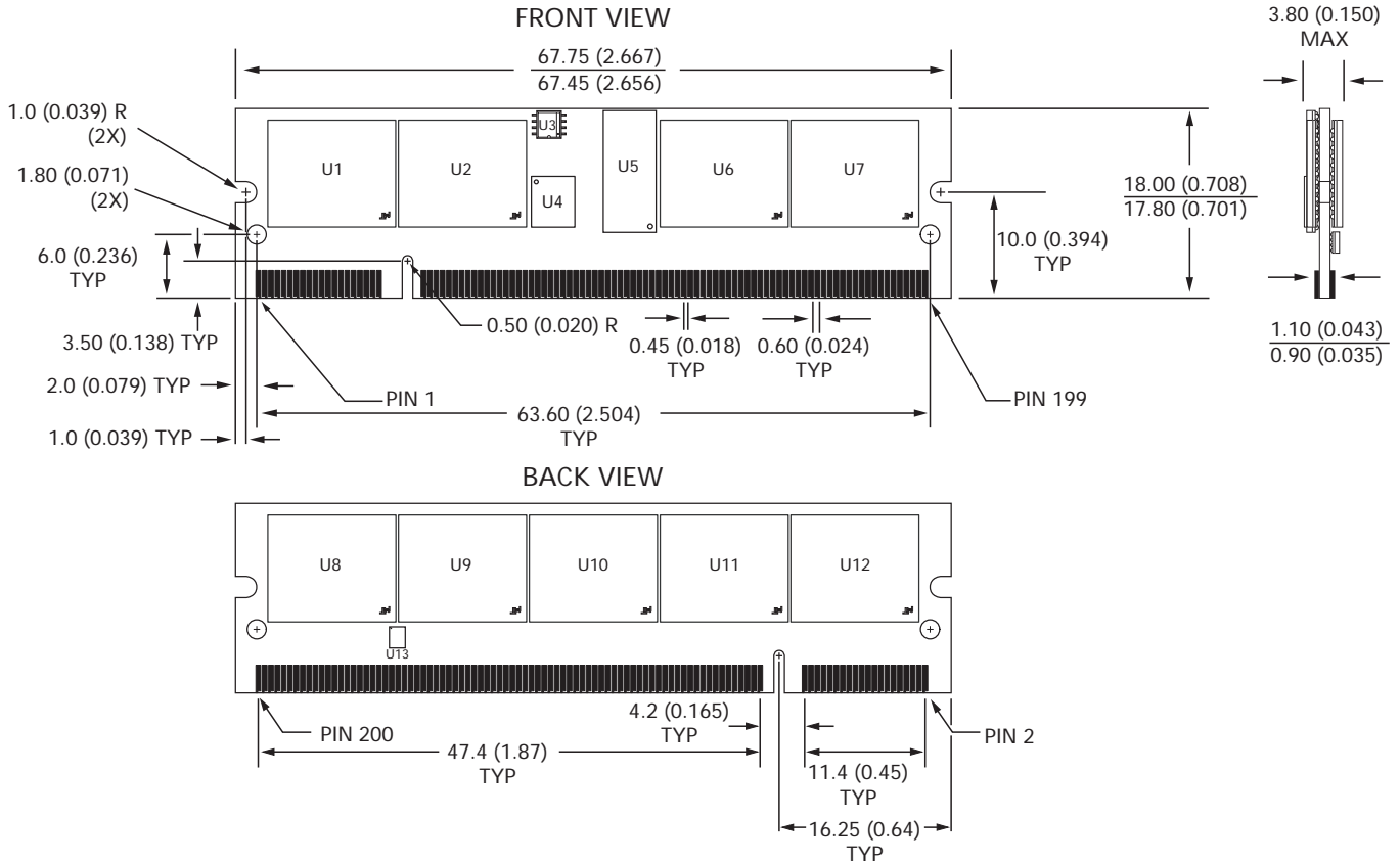
Figure 5: 200-Pin DDR2 VLP SODIMM Dimensions
