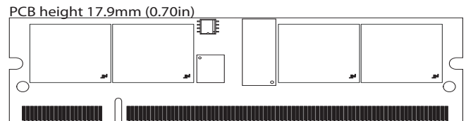
Figure 1: 200-Pin VLP SORDIMM (MO-224)
