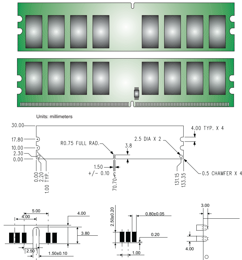
Figure 1: KVR800D2N6/2G 240-Pin DIMM
