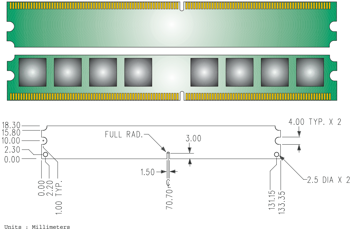
Figure 1: KVR800D2N5K2/2G 240-Pin DIMM Kit
